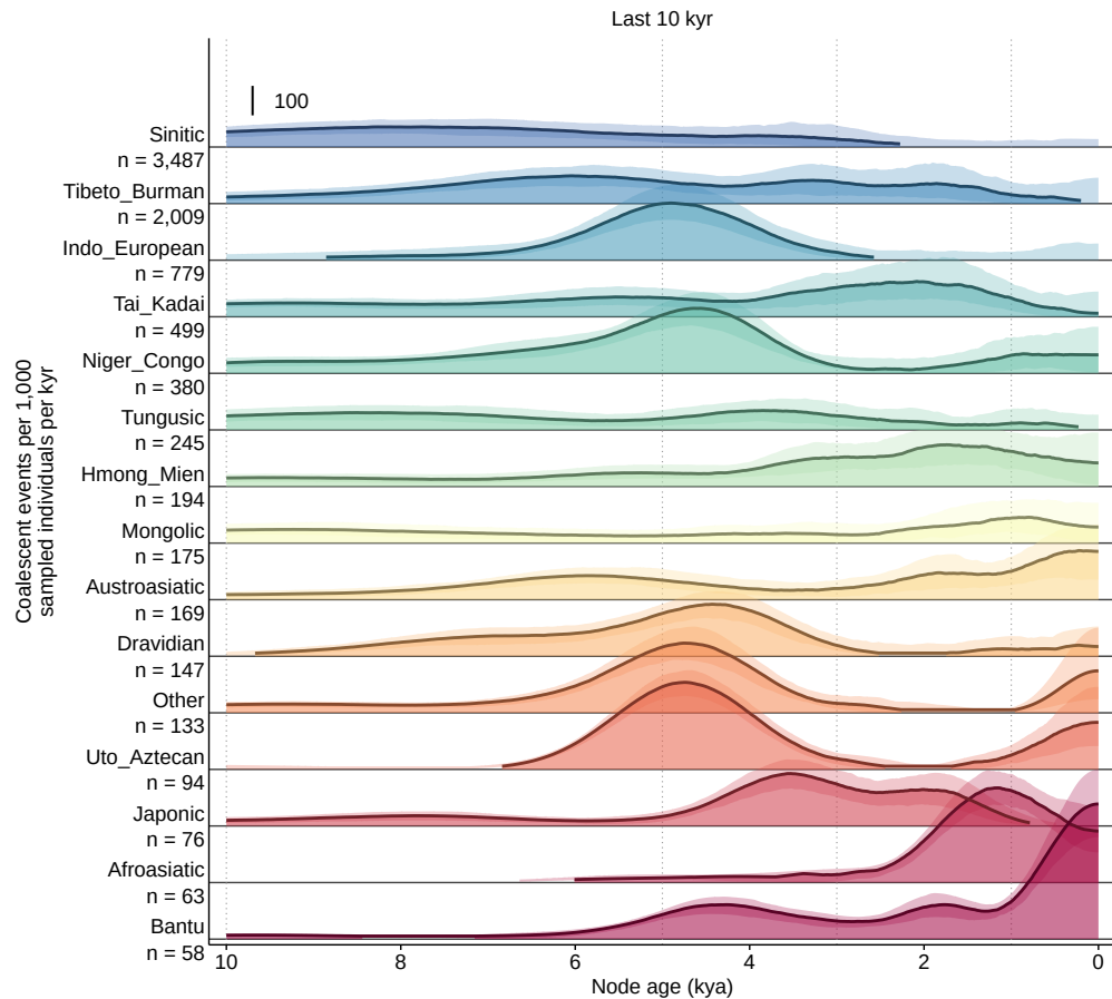
Coalescent event density by Language
