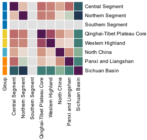
11000-11500 Years — Feature similarity
