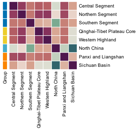
4500-5000 Years — Co-clustering frequency
