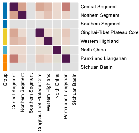
12500-13000 Years — Co-clustering frequency
