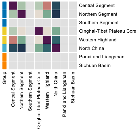
19000-19500 Years — Feature similarity
