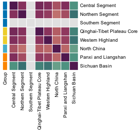
10000-10500 Years — Co-clustering frequency
