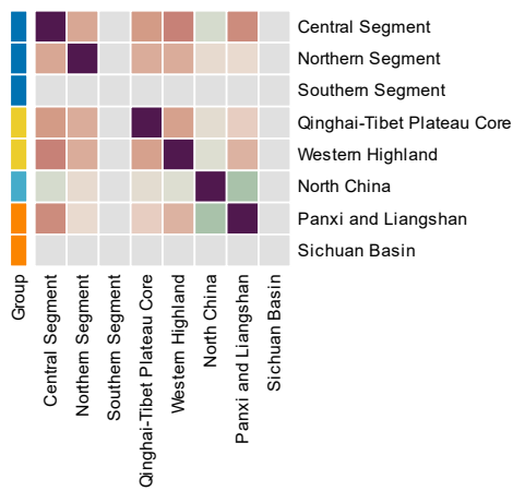
15000-15500 Years — Co-clustering frequency
