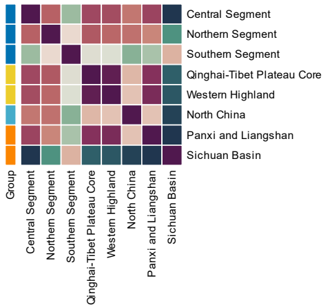
0-500 Years — Feature similarity
