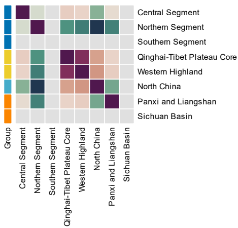
12000-12500 Years — Feature similarity
