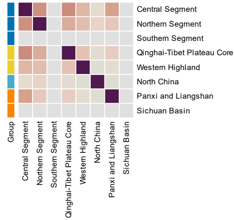
17500-18000 Years — Co-clustering frequency
