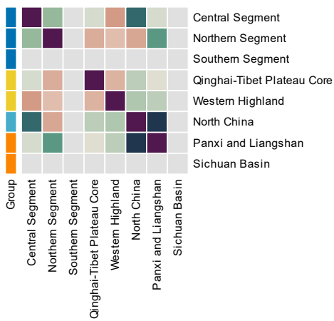
15000-15500 Years — Feature similarity
