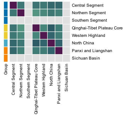
16500-17000 Years — Co-clustering frequency
