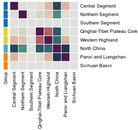
17000-17500 Years — Feature similarity
