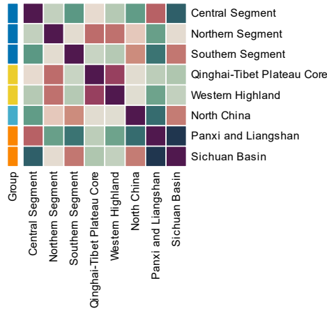
2500-3000 Years — Feature similarity
