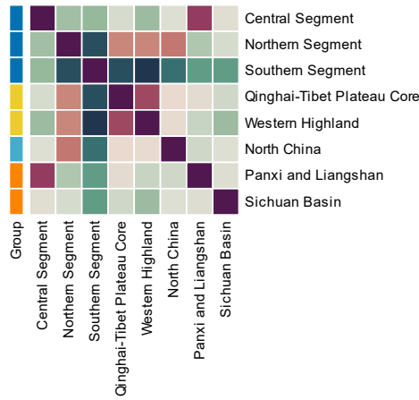
2000-2500 Years — Feature similarity
