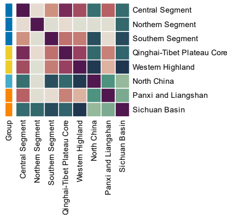
7000-7500 Years — Feature similarity
