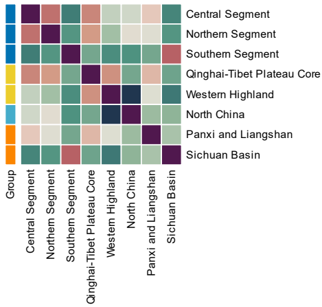
8000-8500 Years — Feature similarity
