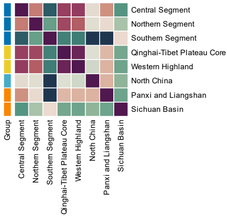
9000-9500 Years — Feature similarity
