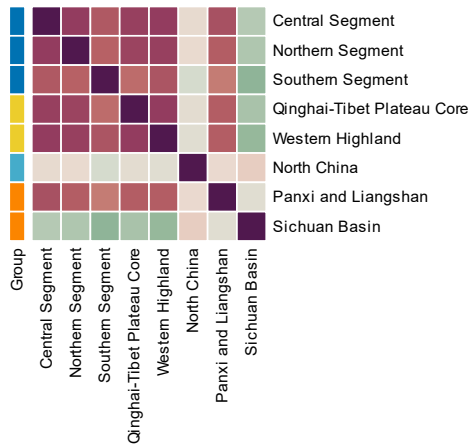
7000-7500 Years — Co-clustering frequency
