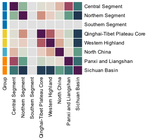
10500-11000 Years — Feature similarity
