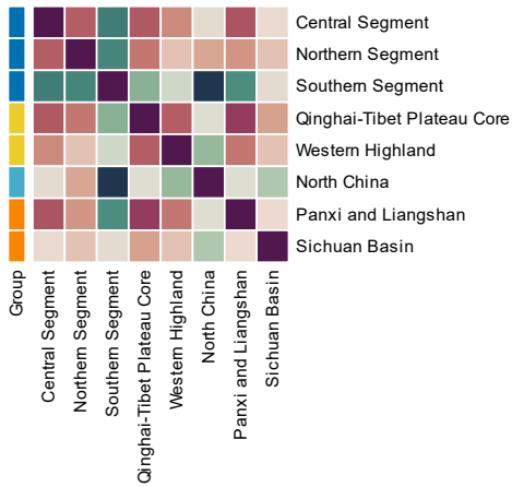
7500-8000 Years — Feature similarity
