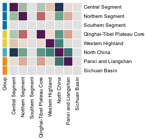
16000-16500 Years — Feature similarity
