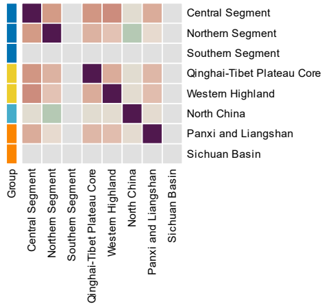
11500-12000 Years — Co-clustering frequency
