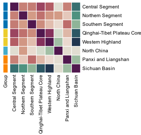
6500-7000 Years — Feature similarity
