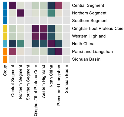
16500-17000 Years — Feature similarity
