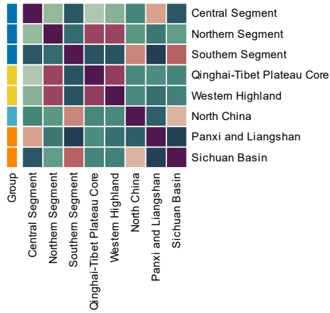
2500-3000 Years — Co-clustering frequency
