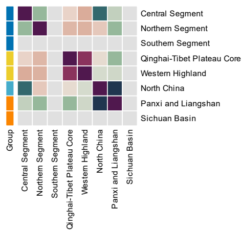
13500-14000 Years — Feature similarity
