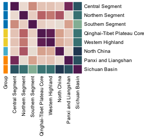
1500-2000 Years — Feature similarity
