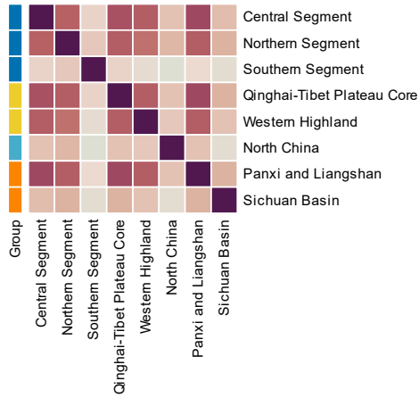
8500-9000 Years — Co-clustering frequency
