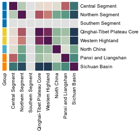
9500-10000 Years — Feature similarity
