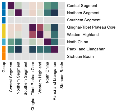
12500-13000 Years — Feature similarity
