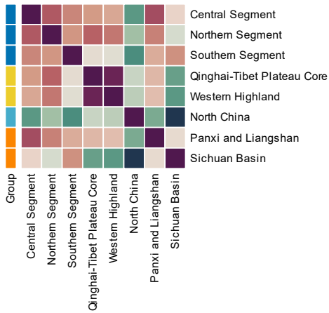
4500-5000 Years — Feature similarity
