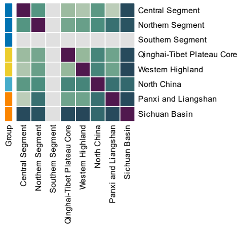
9500-10000 Years — Co-clustering frequency
