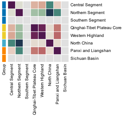
11500-12000 Years — Feature similarity
