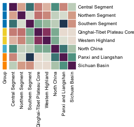
3000-3500 Years — Feature similarity
