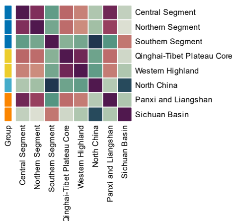
4000-4500 Years — Feature similarity
