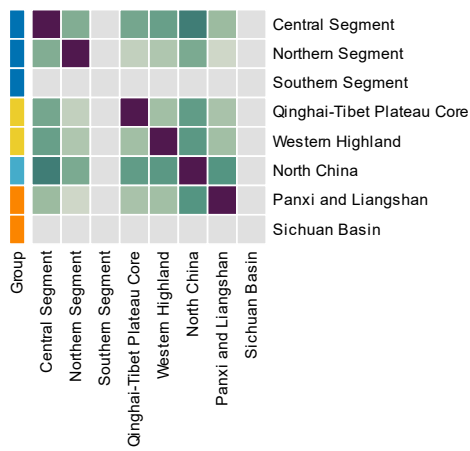
15500-16000 Years — Co-clustering frequency
