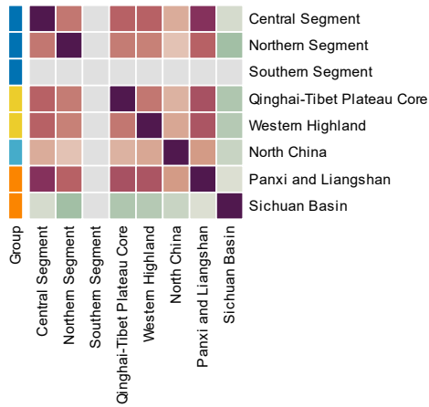
10500-11000 Years — Co-clustering frequency
