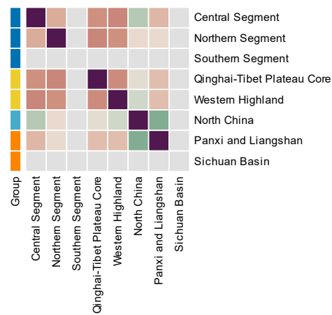
14500-15000 Years — Co-clustering frequency
