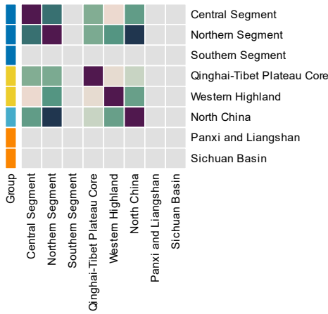
18500-19000 Years — Feature similarity
