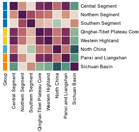
500-1000 Years — Co-clustering frequency
