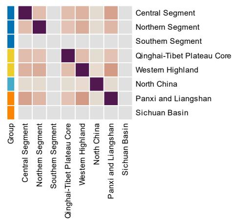
13500-14000 Years — Co-clustering frequency
