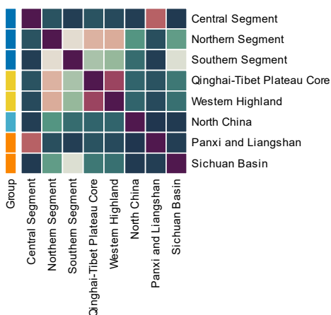
3500-4000 Years — Co-clustering frequency
