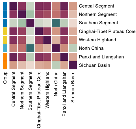
7500-8000 Years — Co-clustering frequency
