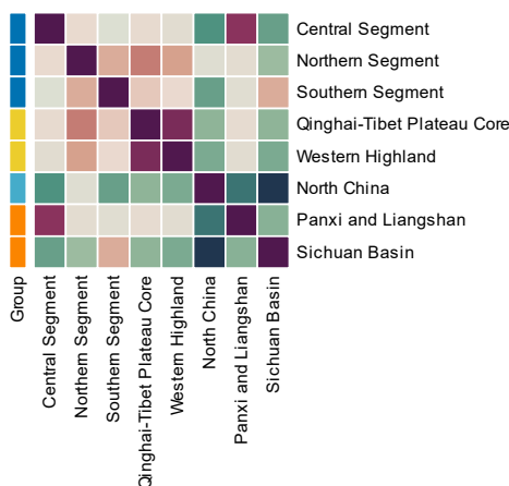
3500-4000 Years — Feature similarity
