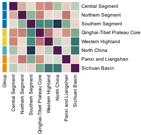
5000-5500 Years — Feature similarity
