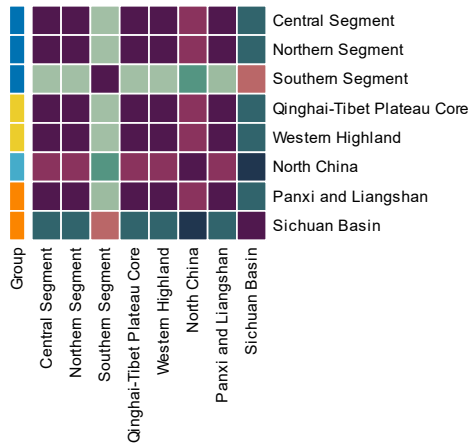
0-500 Years — Co-clustering frequency
