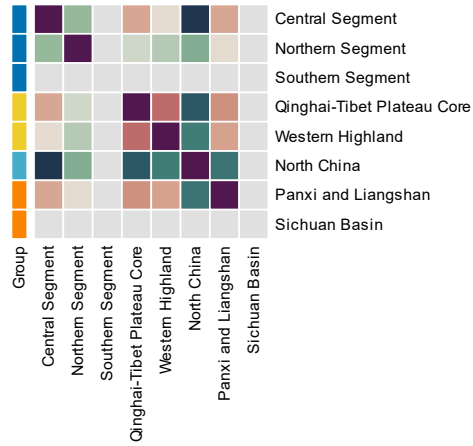
17500-18000 Years — Feature similarity
