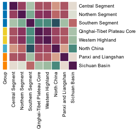
5000-5500 Years — Co-clustering frequency
