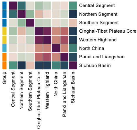
1000-1500 Years — Feature similarity
