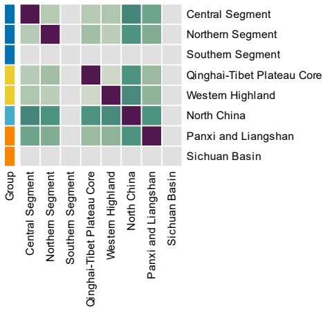
18000-18500 Years — Co-clustering frequency
