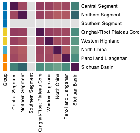
11000-11500 Years — Co-clustering frequency
