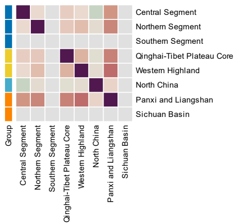
12000-12500 Years — Co-clustering frequency
