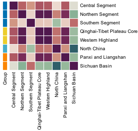
1000-1500 Years — Co-clustering frequency
