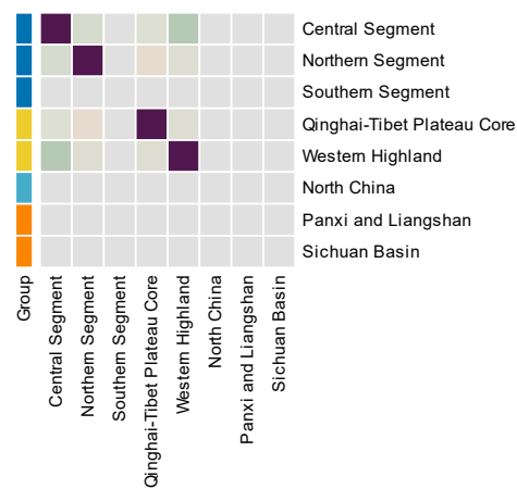
19500-20000 Years — Co-clustering frequency
