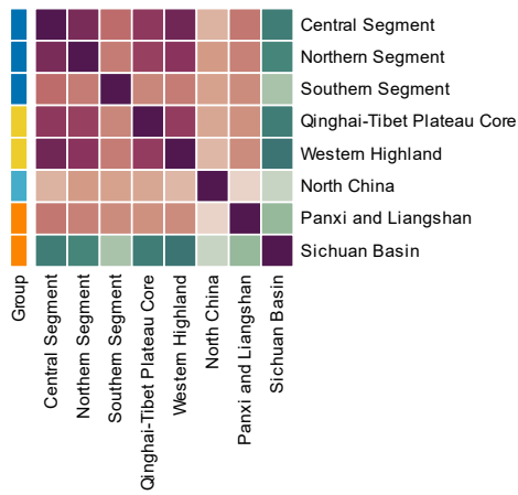
6500-7000 Years — Co-clustering frequency
