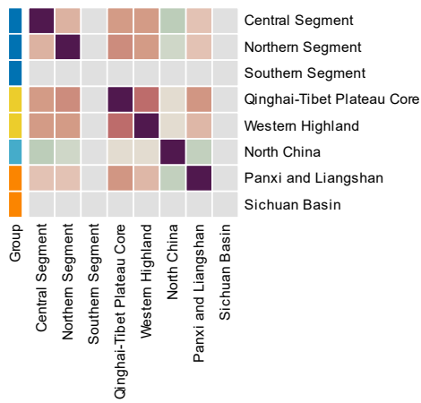
16000-16500 Years — Co-clustering frequency
