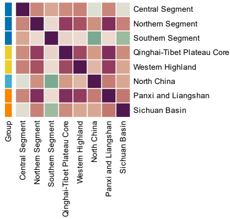
5500-6000 Years — Co-clustering frequency
