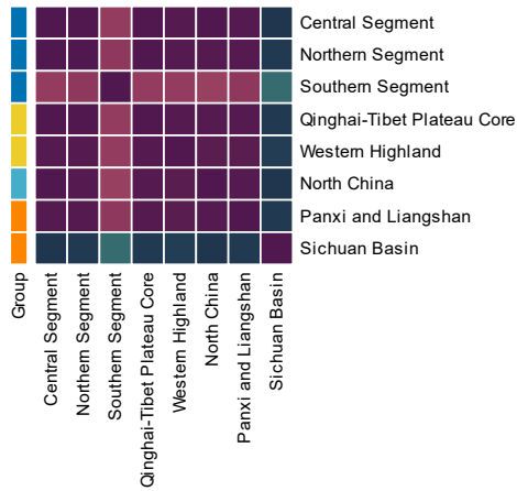
1500-2000 Years — Co-clustering frequency
