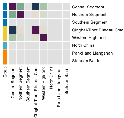
19500-20000 Years — Feature similarity
