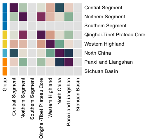
15500-16000 Years — Feature similarity
