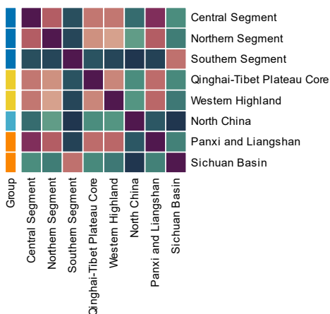
4000-4500 Years — Co-clustering frequency
