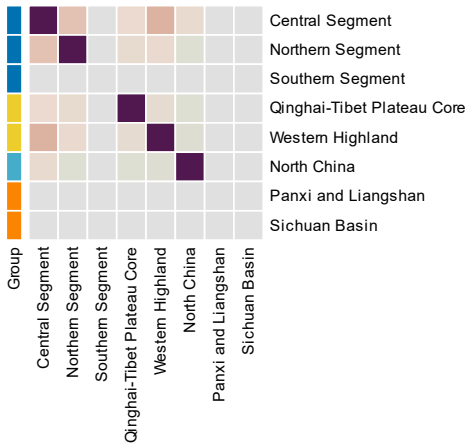
18500-19000 Years — Co-clustering frequency
