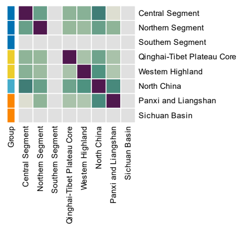
14000-14500 Years — Co-clustering frequency
