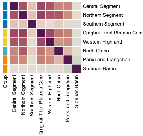
8000-8500 Years — Co-clustering frequency
