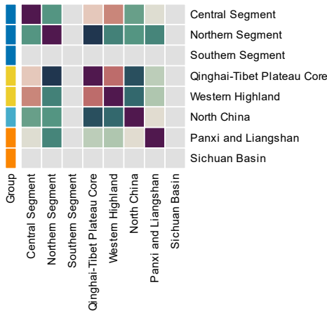
18000-18500 Years — Feature similarity
