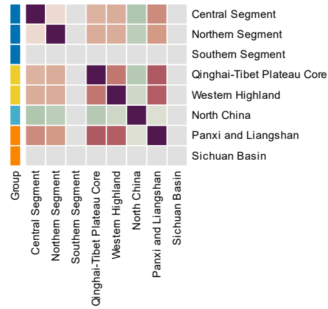
17000-17500 Years — Co-clustering frequency
