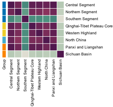
9000-9500 Years — Co-clustering frequency
