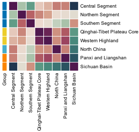
500-1000 Years — Feature similarity
