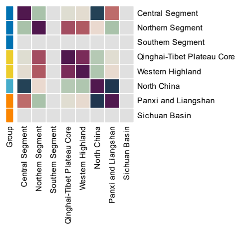
14000-14500 Years — Feature similarity
