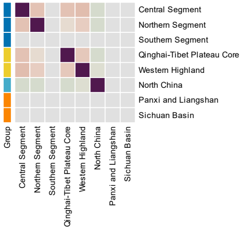
19000-19500 Years — Co-clustering frequency
