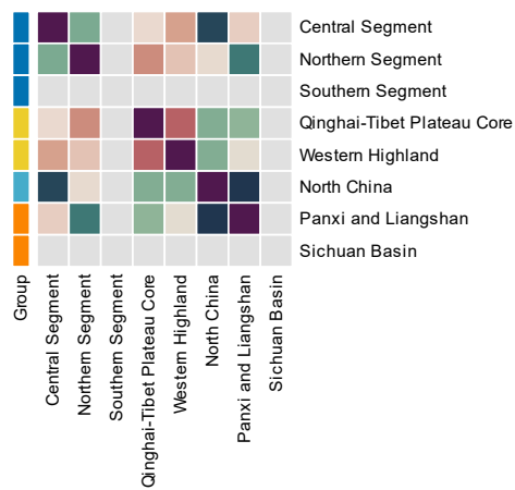
14500-15000 Years — Feature similarity
