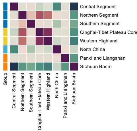
6000-6500 Years — Feature similarity
