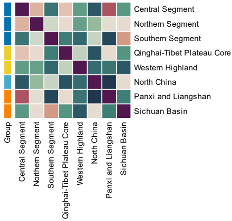
8500-9000 Years — Feature similarity
