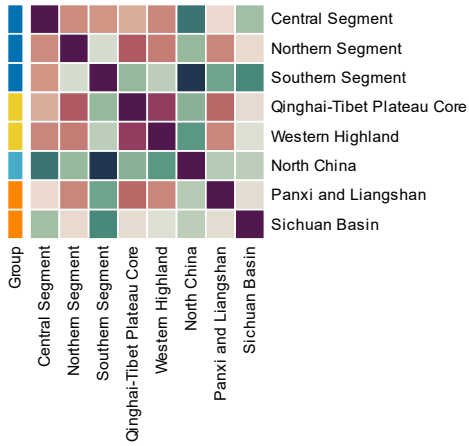
5500-6000 Years — Feature similarity
