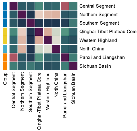
2000-2500 Years — Co-clustering frequency
