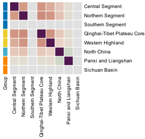
13000-13500 Years — Co-clustering frequency
