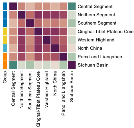
6000-6500 Years — Co-clustering frequency
