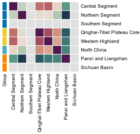
13000-13500 Years — Feature similarity
