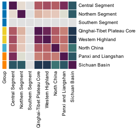
10000-10500 Years — Feature similarity
