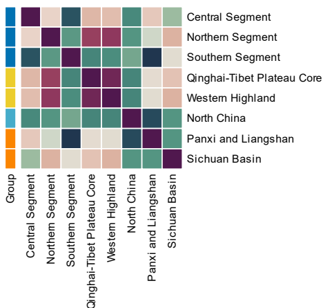
3000-3500 Years — Co-clustering frequency
