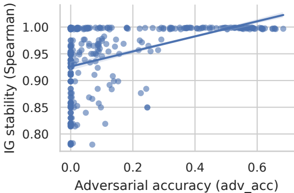
Robustness vs stability (overall)
