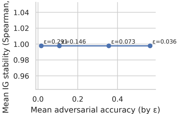
Mean stability vs robustness — FGSM_LP
