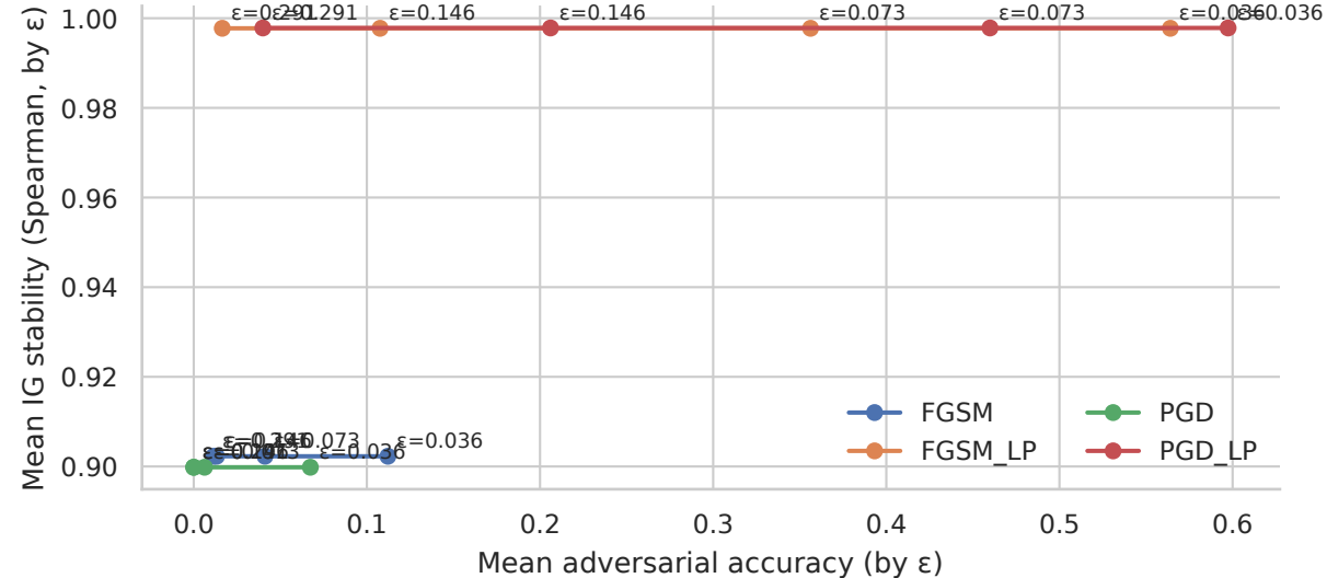
Mean stability vs mean robustness by \epsilon
