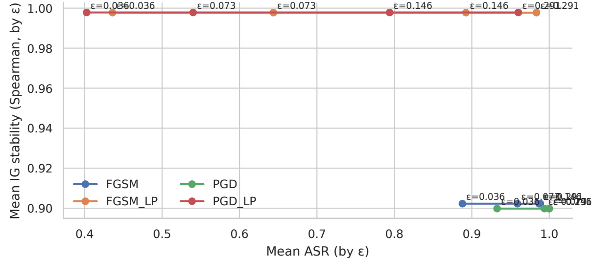
Mean stability vs mean ASR by \epsilon
