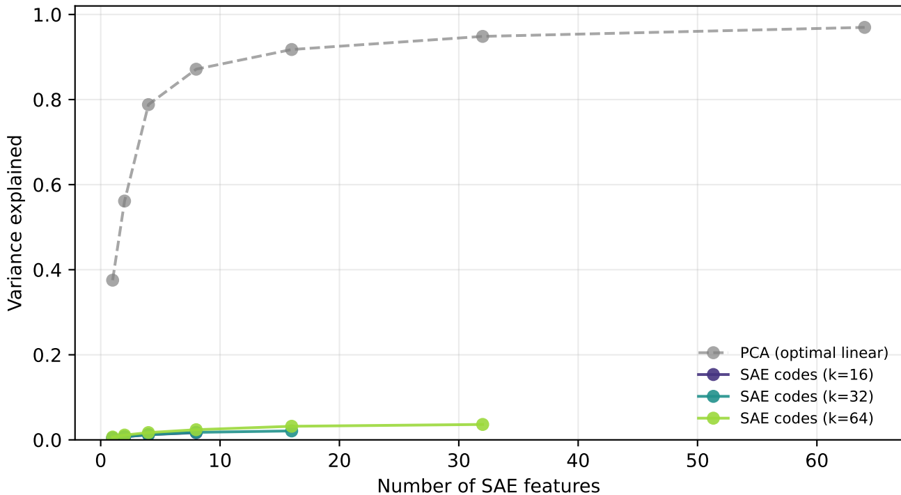
Colors — manifold capture vs. SAE sparsity
