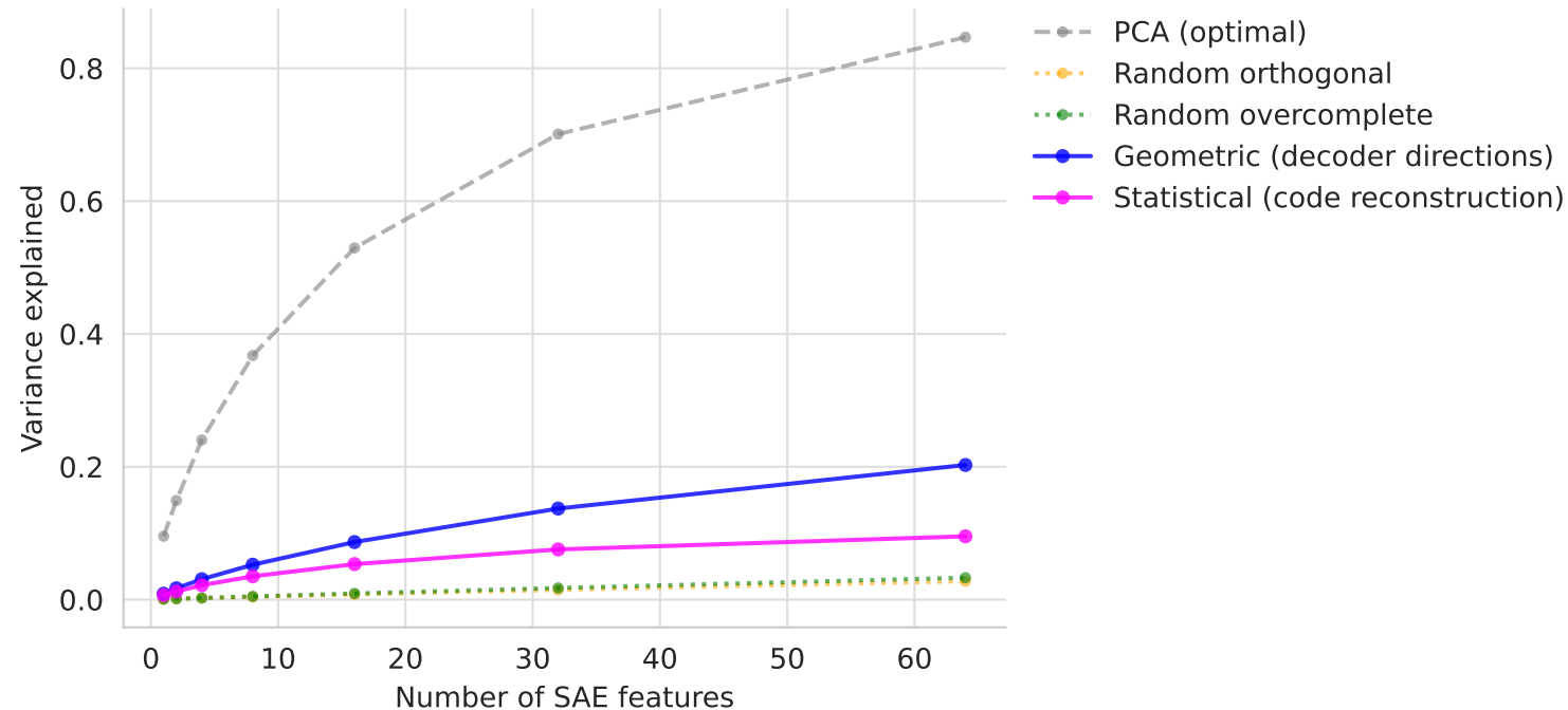
Geography — manifold reconstruction
