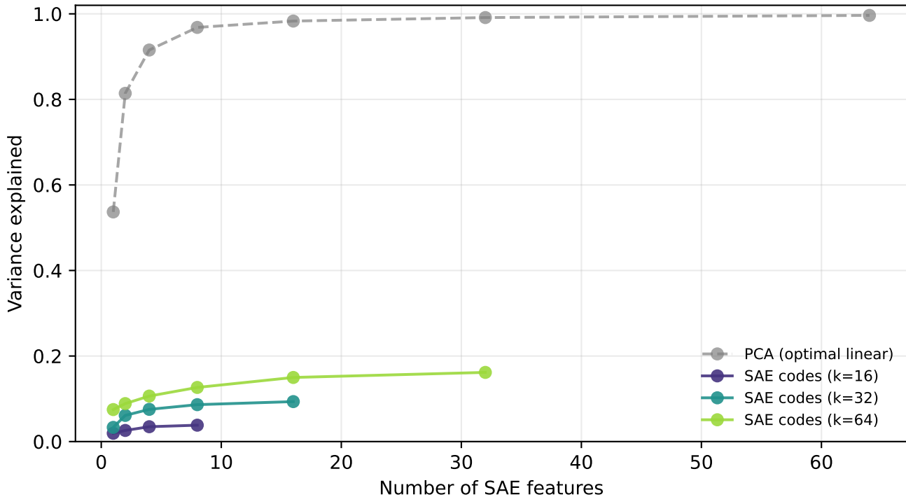
Temperature — manifold capture vs. SAE sparsity
