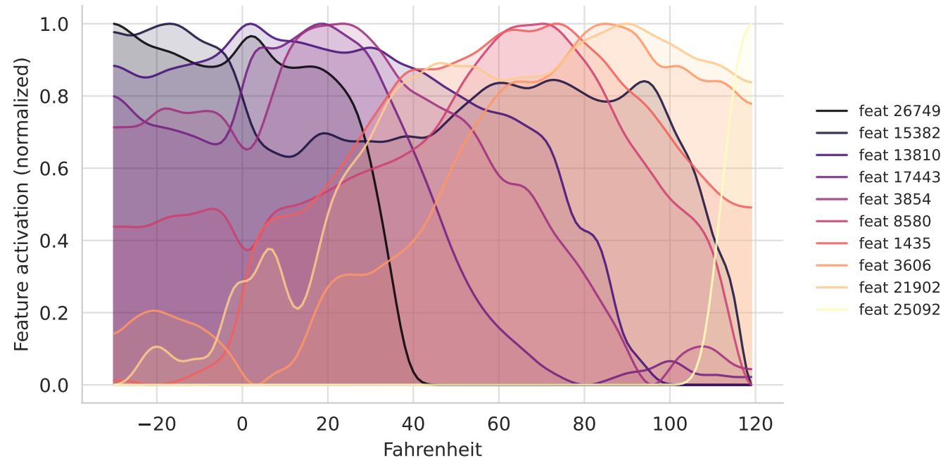
Temperature — feature tuning curves (top 10)
