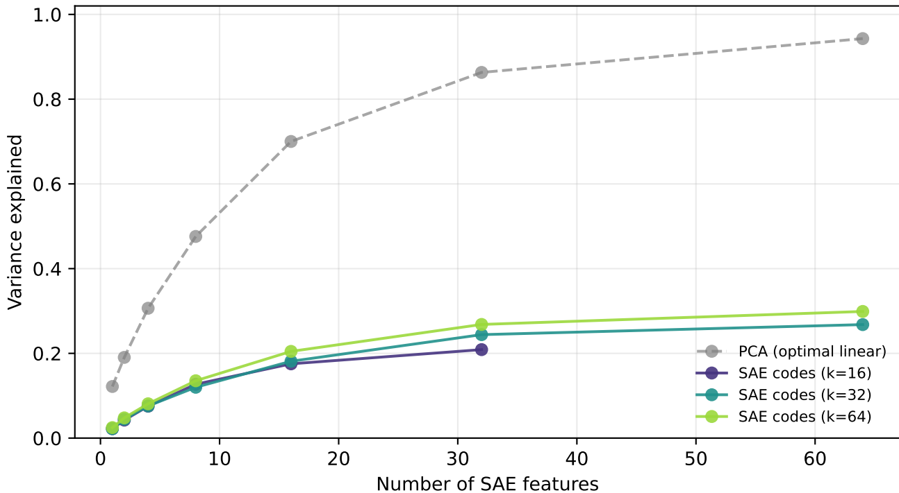
Years — manifold capture vs. SAE sparsity
