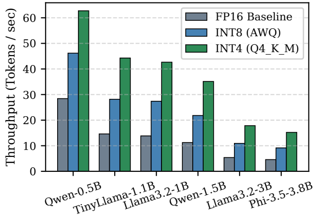
(a) Inference Throughput (Jetson Orin Nano)
