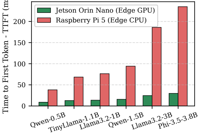
(b) Prompt Evaluation Latency (INT4)
