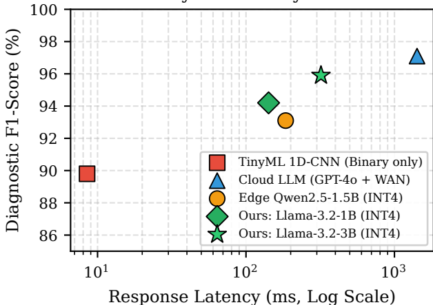
Accuracy vs. Latency Trade-Off
