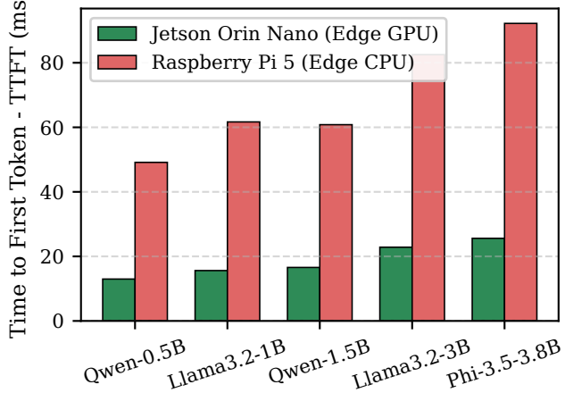
(b) Prompt Evaluation Latency (INT4)
