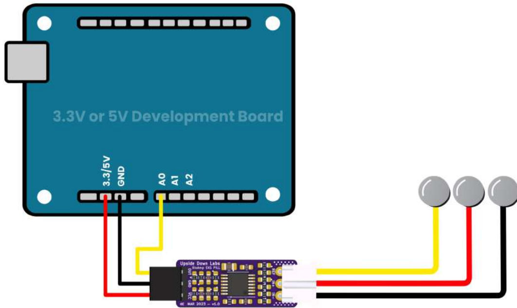
Fig. 7: Complete assembly of BioAmp EXG Pill, Arduino, and BioAmp Cable v3
