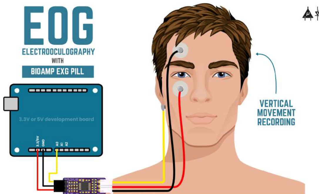
Fig. 13: Vertical EOG Placement
