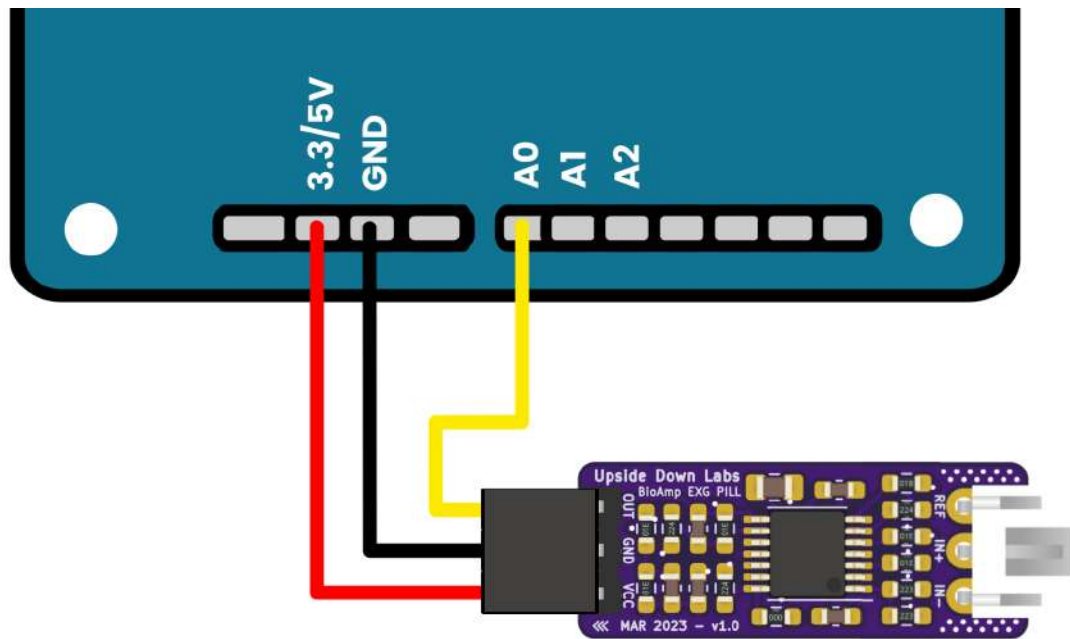
Fig. 5: Connections with Arduino UNO Development Boards
