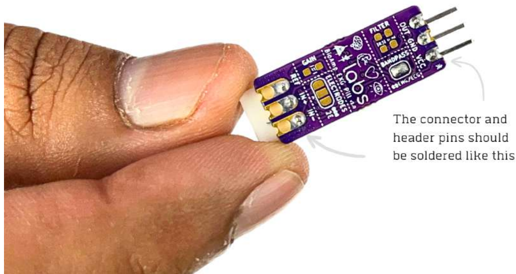
Fig. 3: After soldering, BioAmp EXG Pill should look like this
