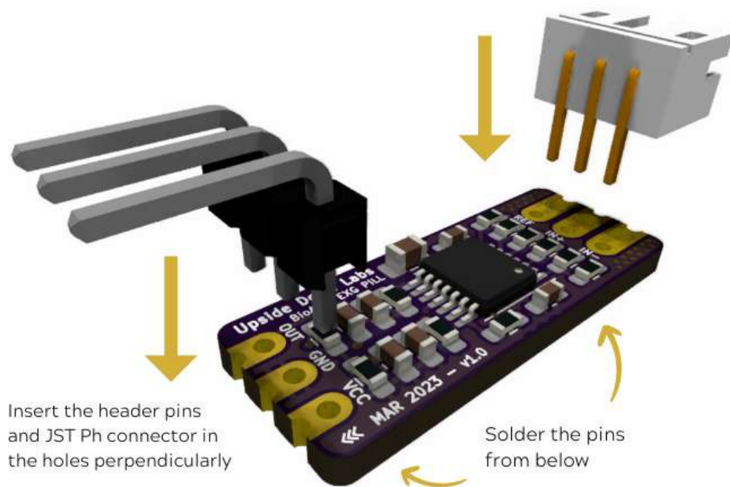
Fig. 2: Soldering the connector & header pins on BioAmp EXG Pill
