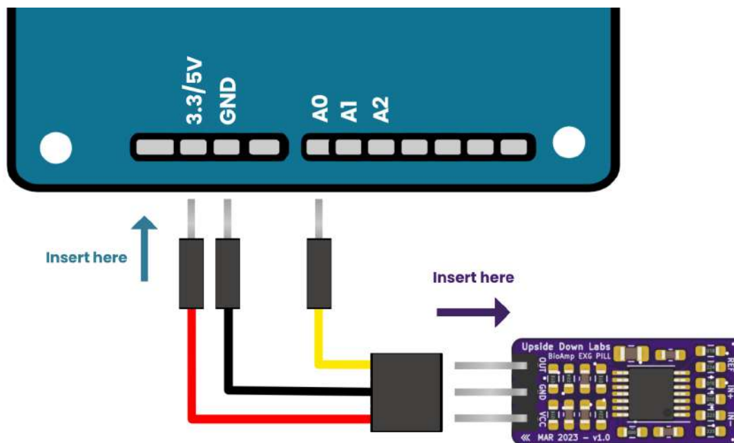
Fig. 4: Wiring diagram for VCC, GND, and OUT Connections with Arduino UNO
