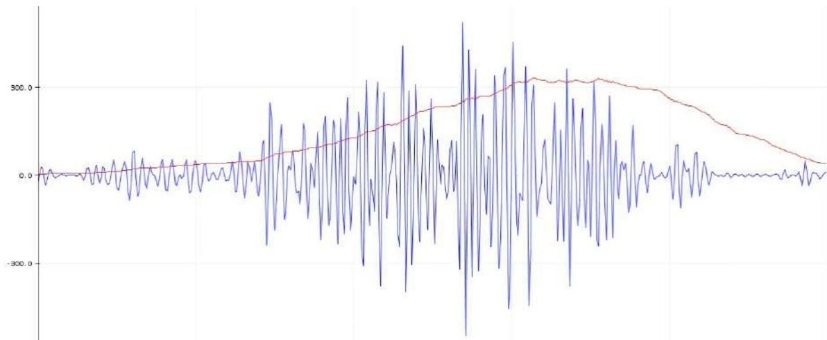
Fig. 9: Visualizing EMG signals on Arduino IDE v1.8.x
