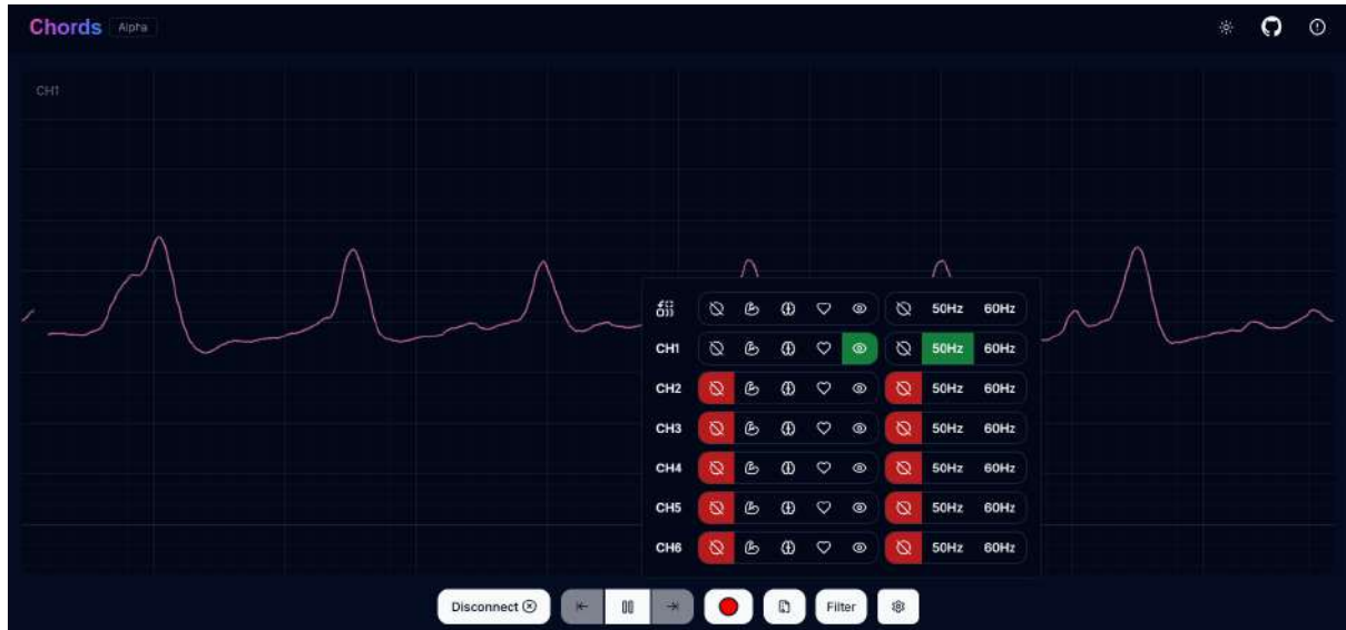
Fig. 14: Visualizing EOG signals on Chords Web
