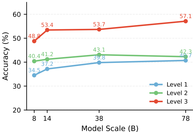
InternVL3 Scale Curve by Level (CoT)
