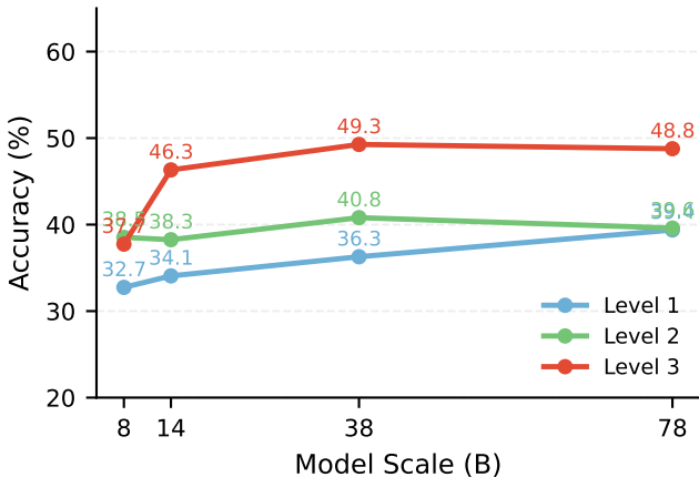
InternVL3 Scale Curve by Level (NoCoT)
