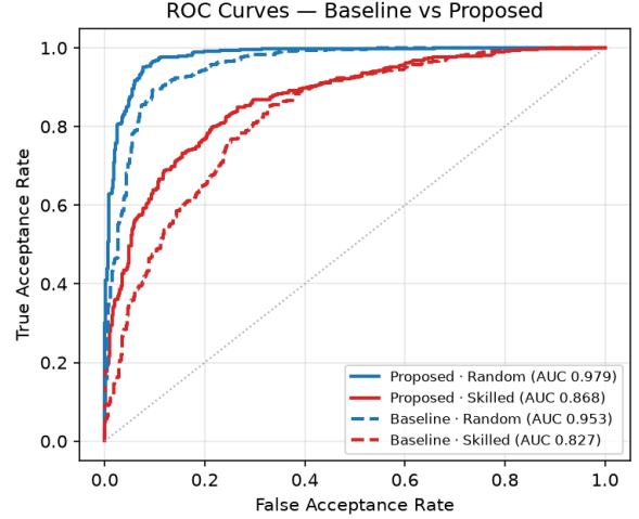
Fig. 5. ROC curves for the baseline and the proposed model, per attack scenario.
