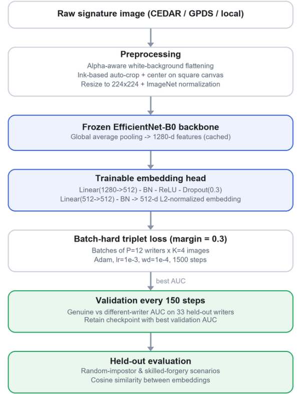
Fig. 2. System flowchart of the proposed pipeline.
