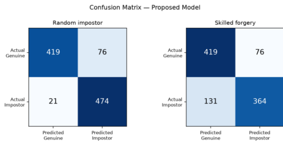
Fig. 7. Confusion matrix of the proposed model for the random-impostor and skilled-forgery scenarios.
