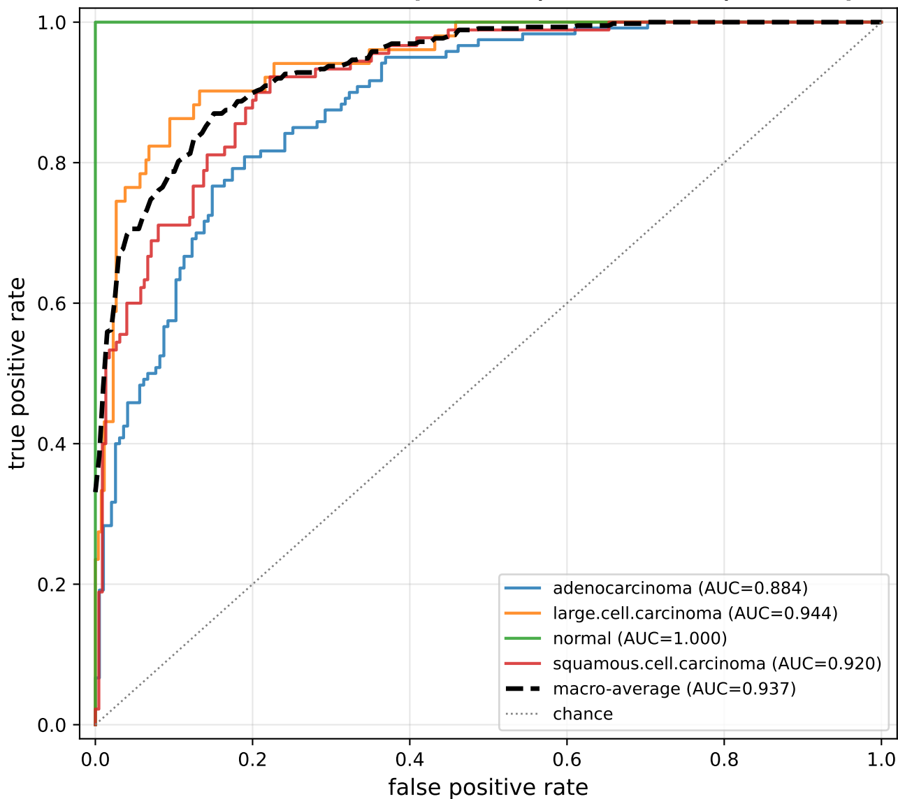
VGG16 - ROC curve (internal, one-vs-rest, 4-class)
