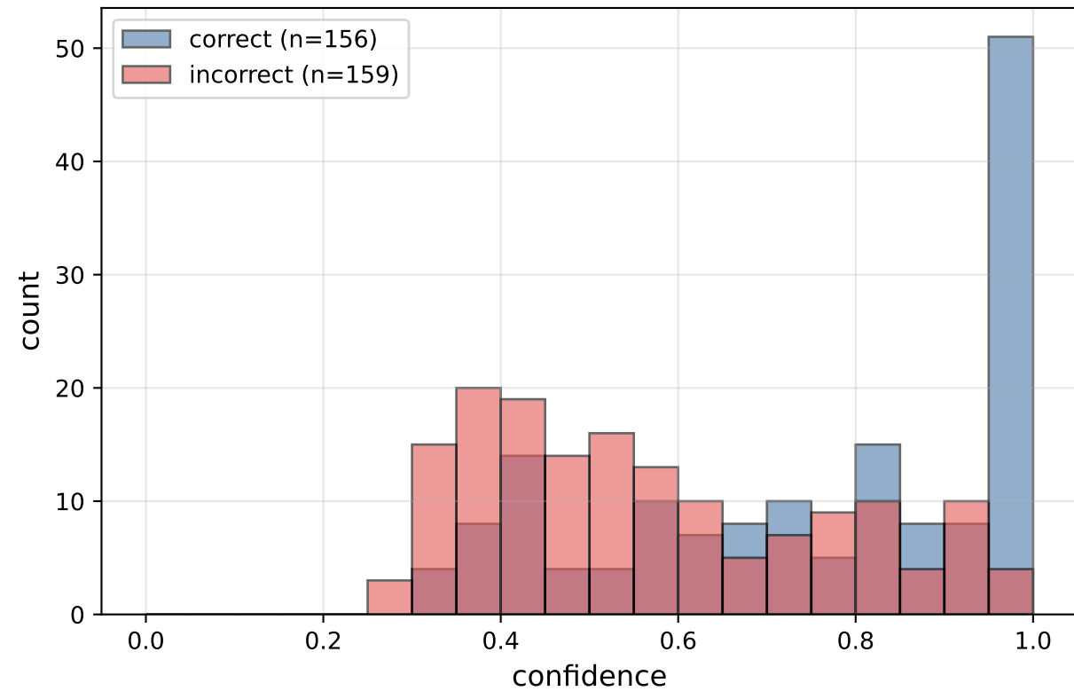
MiniConvNet
