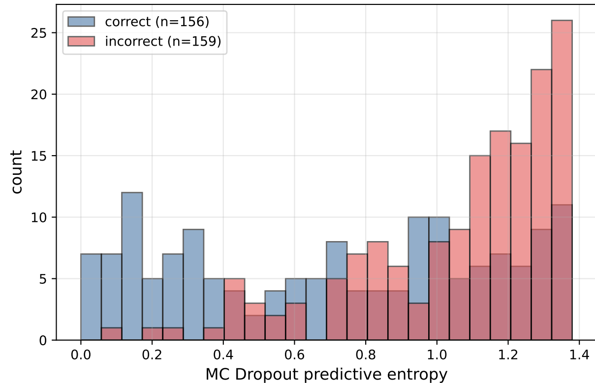
MiniConvNet
