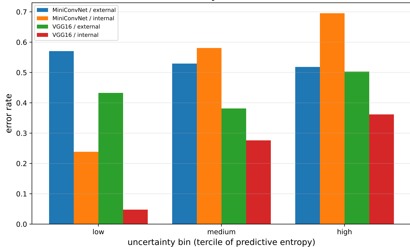
Uncertainty vs error rate
