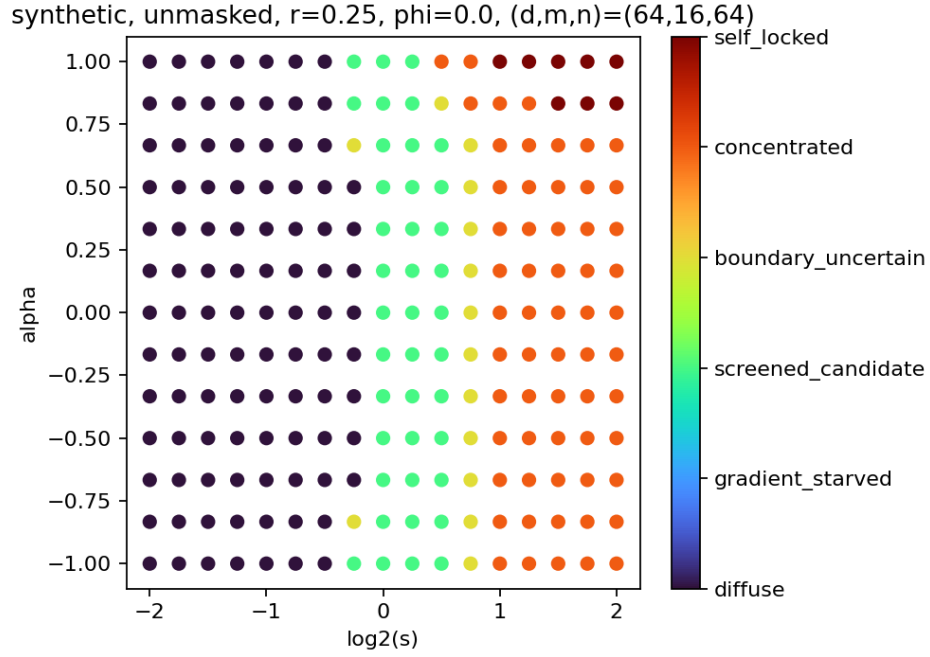
Figure 6.7: Original turbo-colormap scatter from exp1b/run.py analyze.
