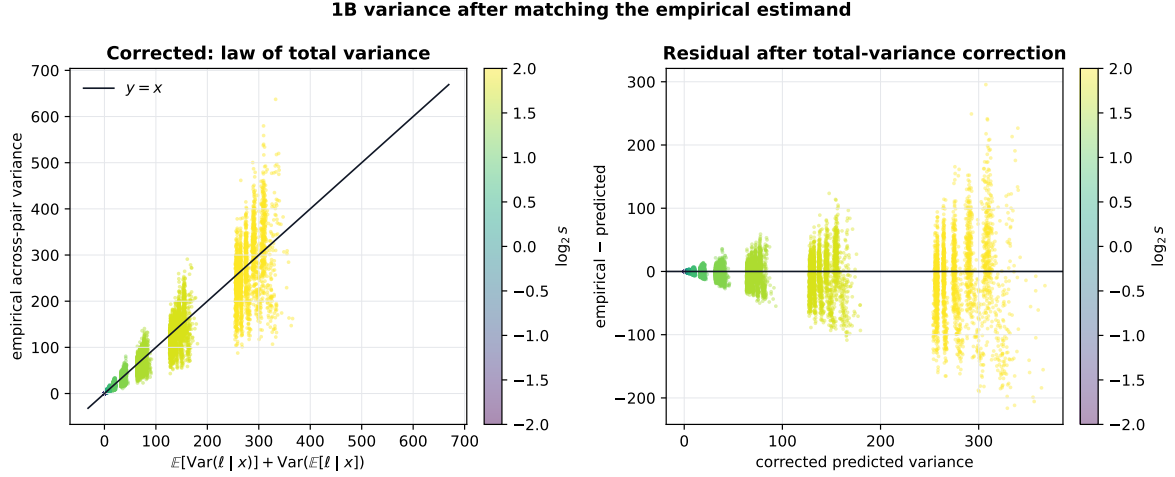
Figure 6.2: Same empirical variance after adding \text{Var}_{ij}(\mathbb{E}[\ell_{ij} \mid x]) . Residuals are closer to centered by scale; remaining error is heteroscedastic single-draw noise, not 1A-style 10^{-2} Monte Carlo error.
