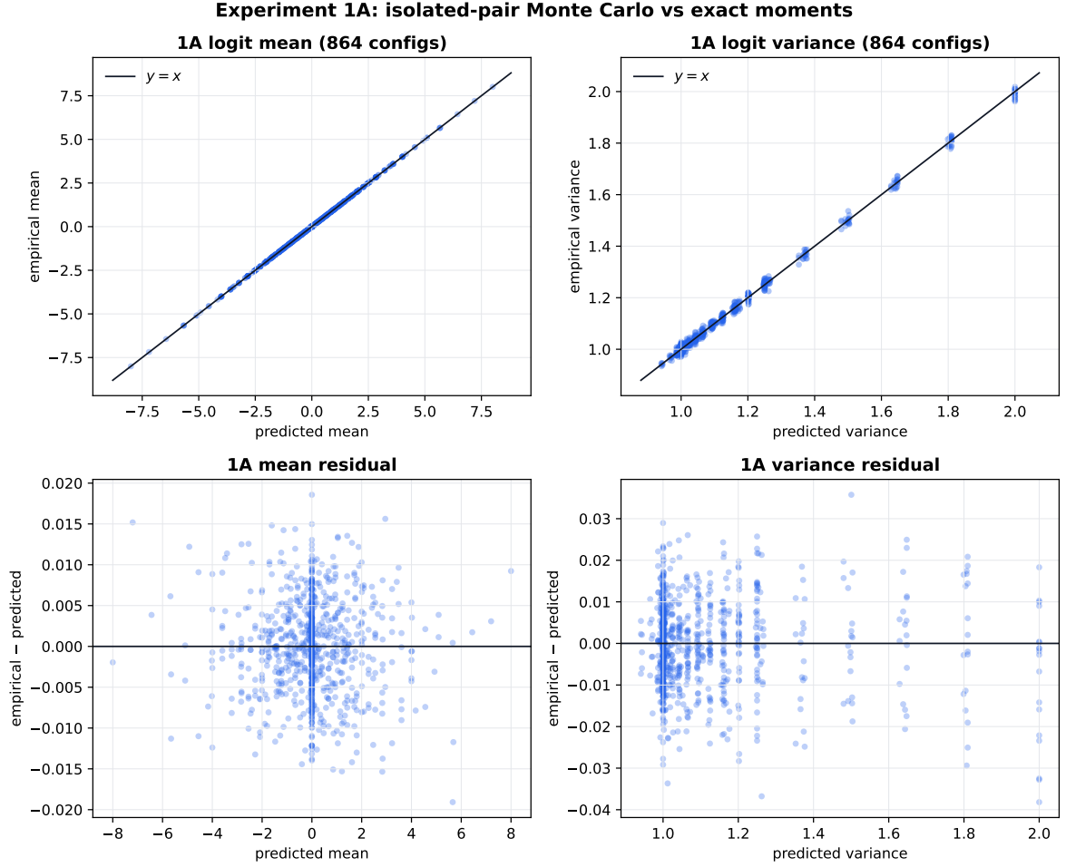
Figure 4.1: Experiment 1A: isolated-pair Monte Carlo moments versus exact theory. Residuals are centered at zero with magnitude \sim 10^{-2} , matching the preregistered precision gate.
