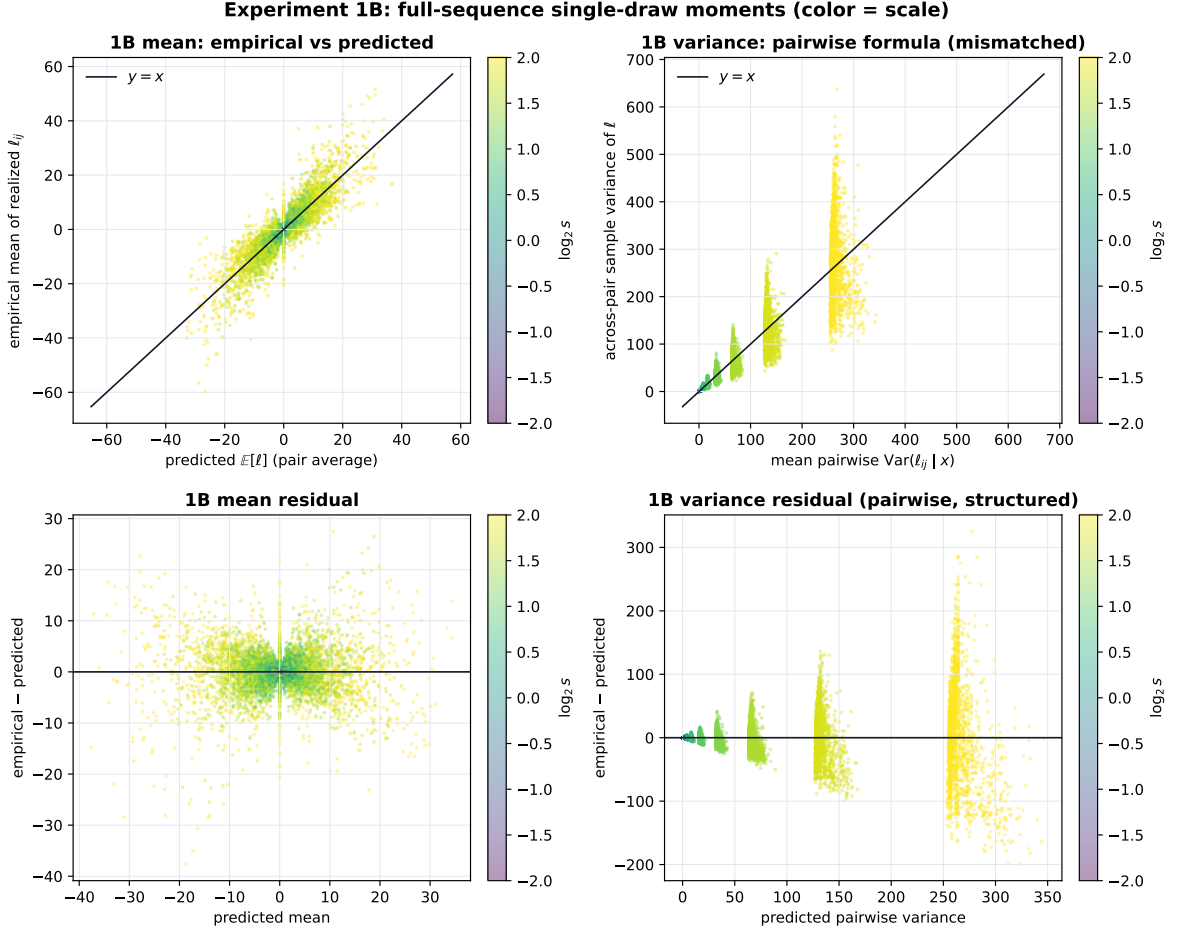
Figure 6.1: 1B single-draw diagnostics. Left: mean is approximately unbiased with heteroscedastic scatter. Right: empirical across-pair variance vs. mean pairwise conditional variance—mismatched estimands, discrete s -bands, large residuals. Color is \log_2 s .
