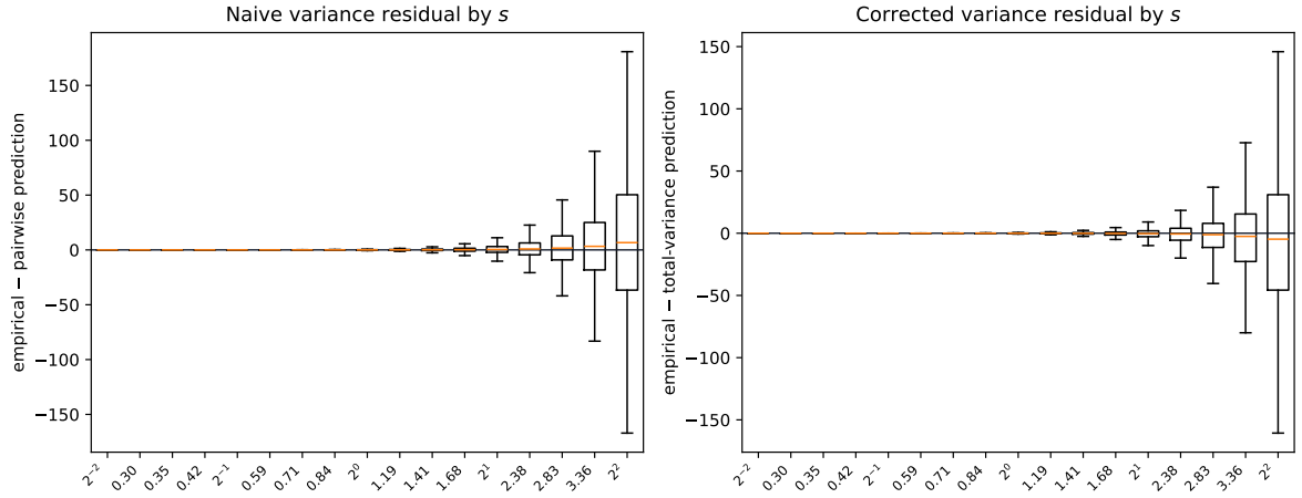
Figure 6.3: Variance residuals boxed by s . Naive pairwise residuals fan out and shift with scale; the total-variance correction recenters medians. Whiskers at s = 4 still span \mathcal{O}(10^2) .
