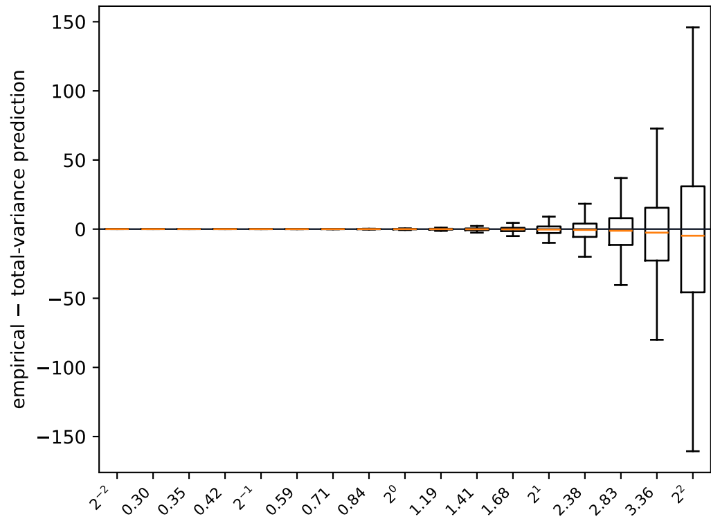
Corrected variance residual by s
