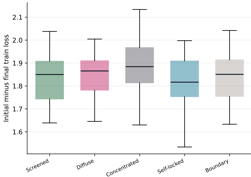
Associative recall
