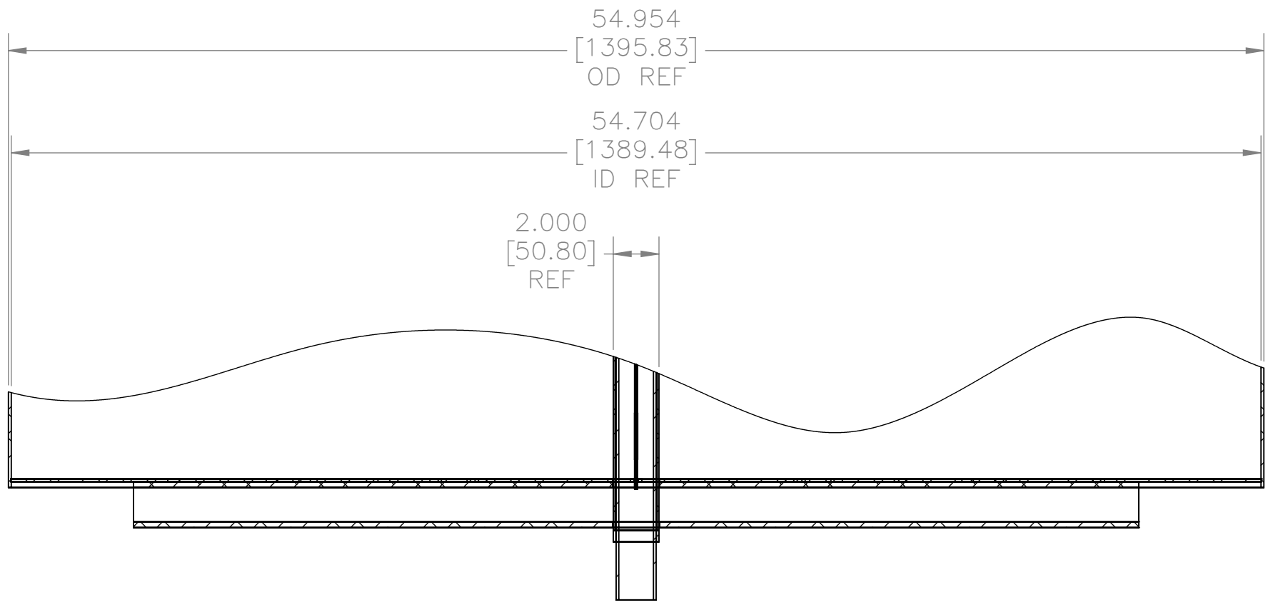
SECTION F-F
