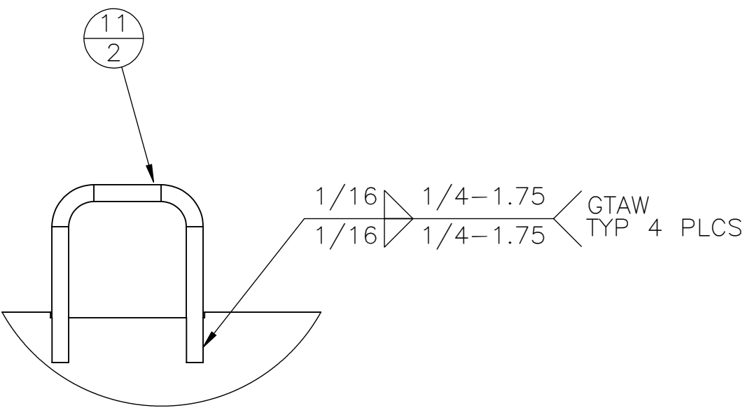
DIVIDER HANDLE DETAIL
