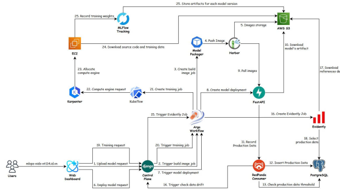
Fig. 3. Prototype workflow of the drift-aware MLOps framework. The Django control plane coordinates upload, packaging, training requests, deployment requests, registry metadata, and drift checks. The FastAPI data plane serves model predictions and emits production logs through Redpanda/PostgreSQL, while Argo/Kubeflow, object storage, Harbor, MLflow, Evidently, and Karpenter-backed compute are used as supporting services where configured.
