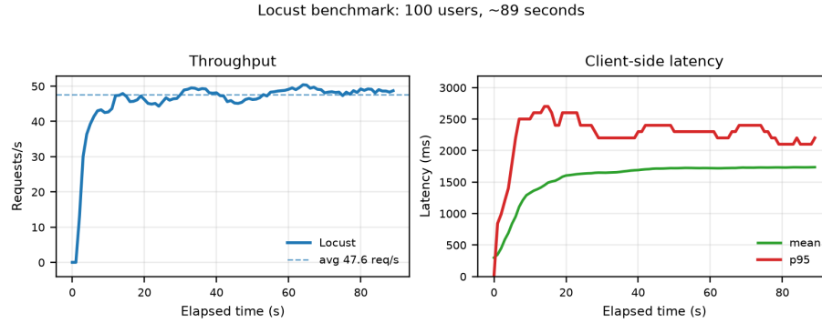
Fig. 4. Prototype serving benchmark with 100 Locust users over an approximately 89-second replay window. Throughput and latency are measured from Locust’s client-side history during the benchmark.
