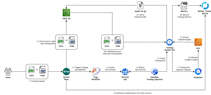
Fig. 3. Training pipeline: the control plane submits a Kubeflow PyTorchJob via Argo Workflows; the runner executes on Karpenter-provisioned EC2 nodes and uploads the resulting artifact to S3, with optional MLflow metric tracking.
