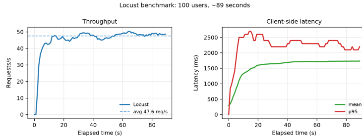
Fig. 7. Bounded prototype serving replay: 100 Locust users, \approx 89 -second window.
