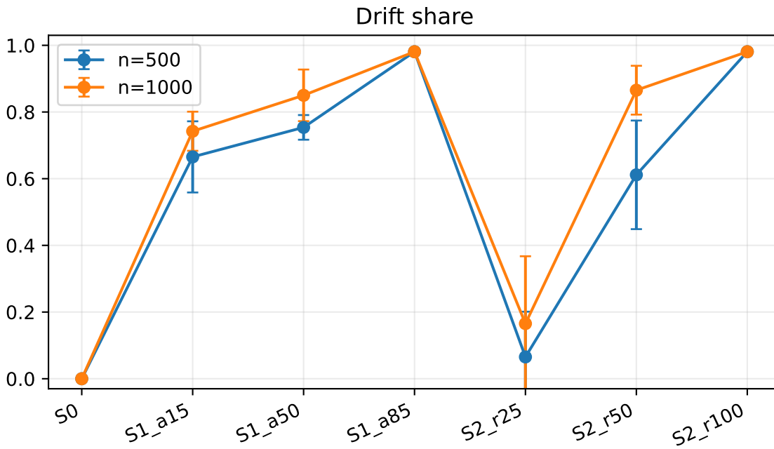
Fixed model: controlled shift; mean \pm sampling SD (5 seeds)
