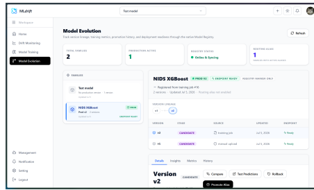
Fig. 4. Model Evolution UI showing version lineage (v1 → v2) and dynamic serving readiness.
