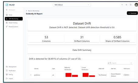
Fig. 5. Evidently AI drift monitoring dashboard showing feature-level drift detection.
