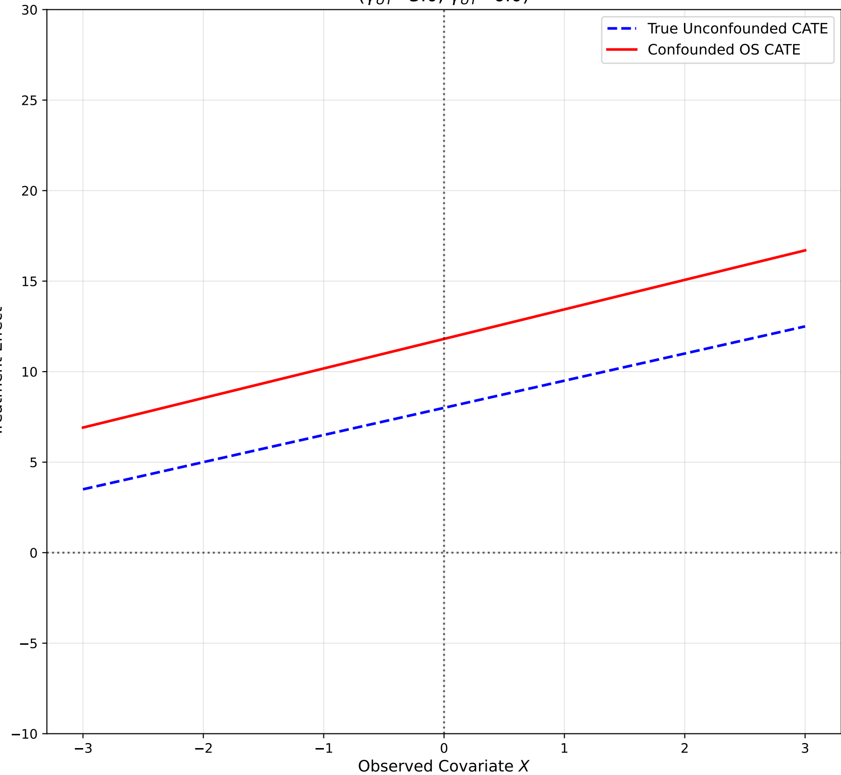
Hidden Confounding in OS ( \gamma_{UY}=3.0 , \gamma_{UT}=6.0 )
