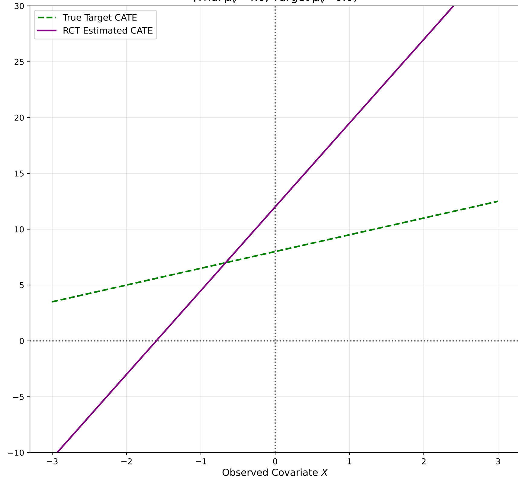
Effect Modification in RCT (Trial \mu_V=4.0 , Target \mu_V=0.0 )
