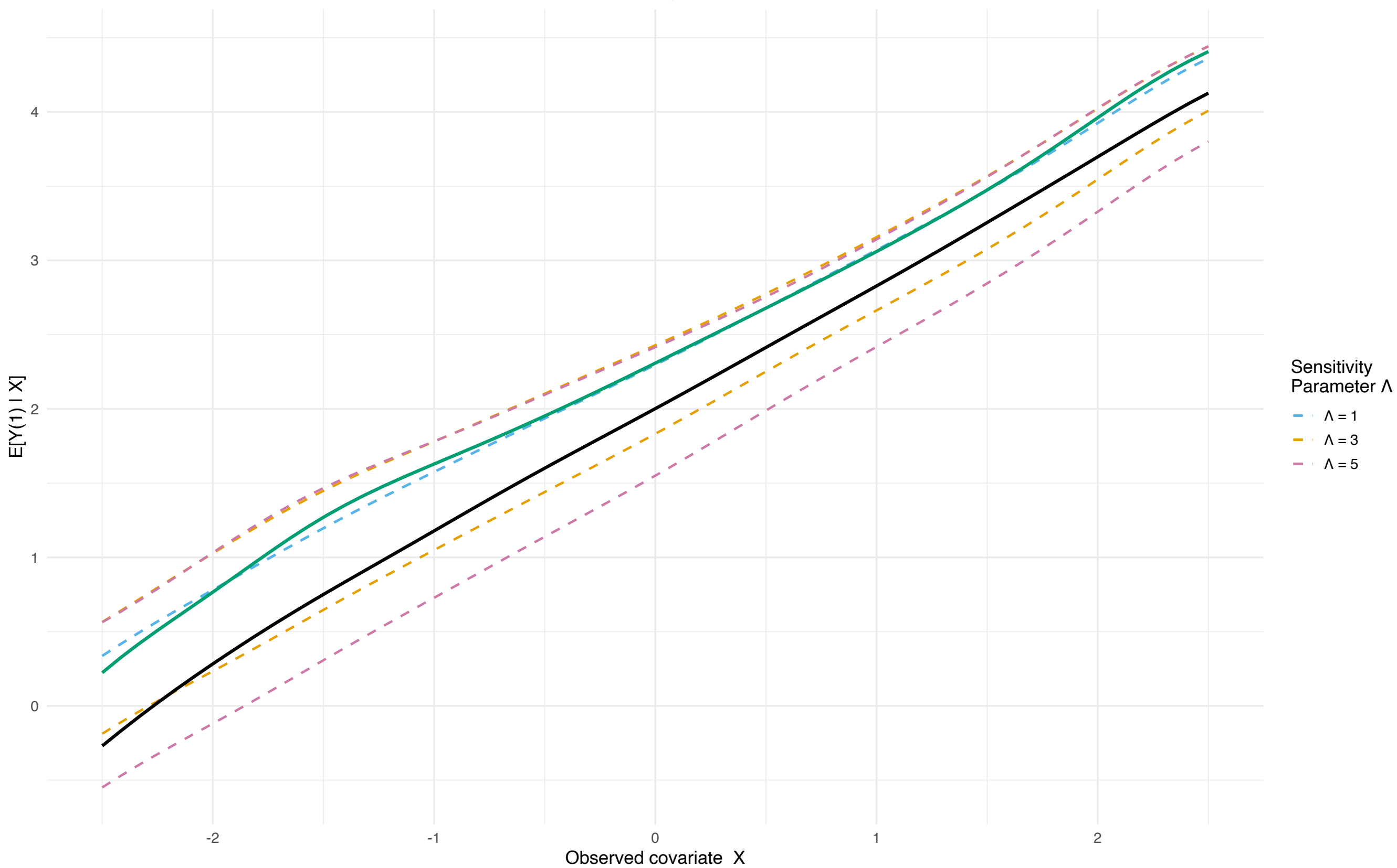
Partial Identification of E[Y(1) | X] under Hidden Confounding
