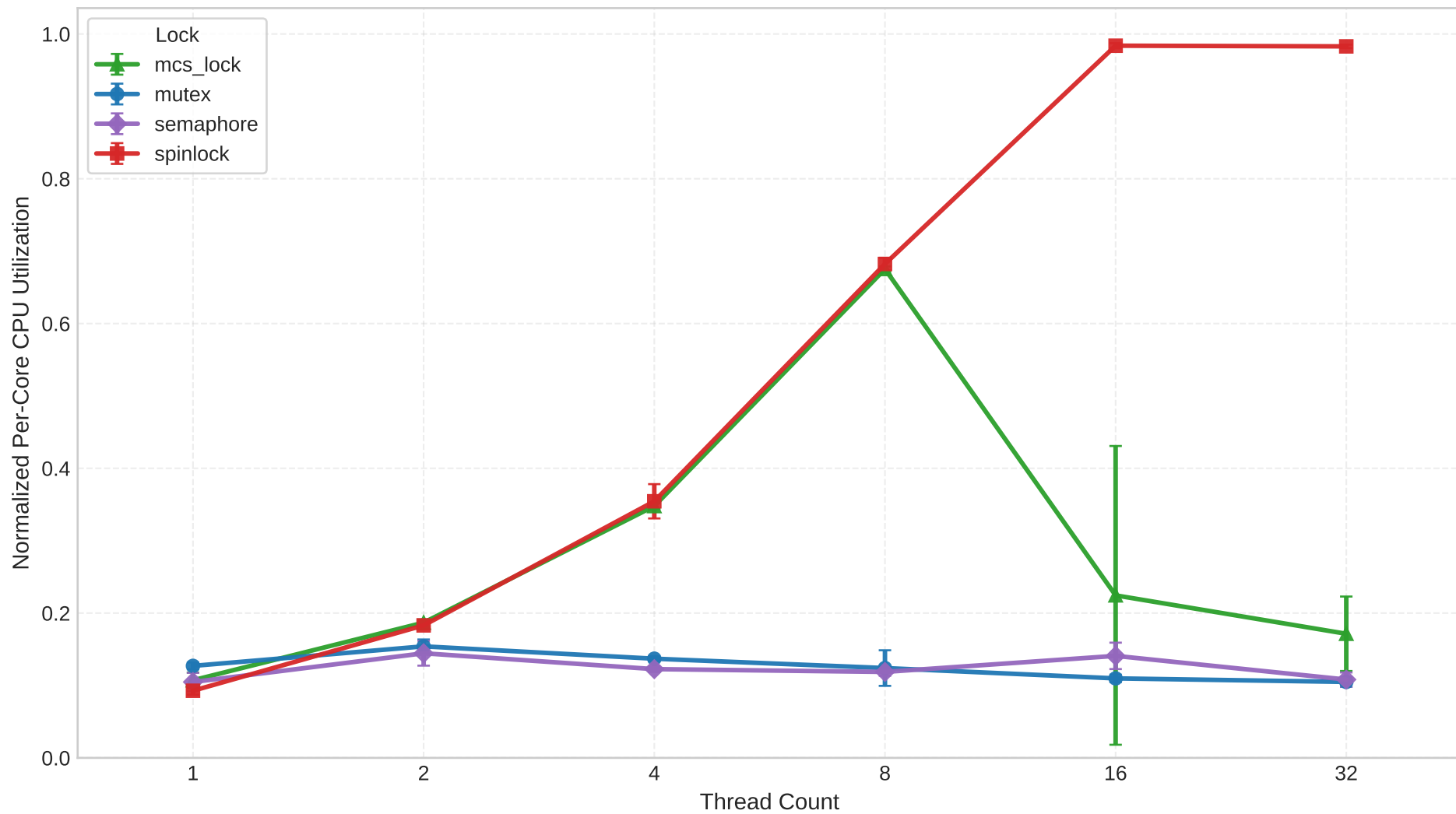
Experiment 1: Normalized Per-Core CPU Utilization vs Thread Count
