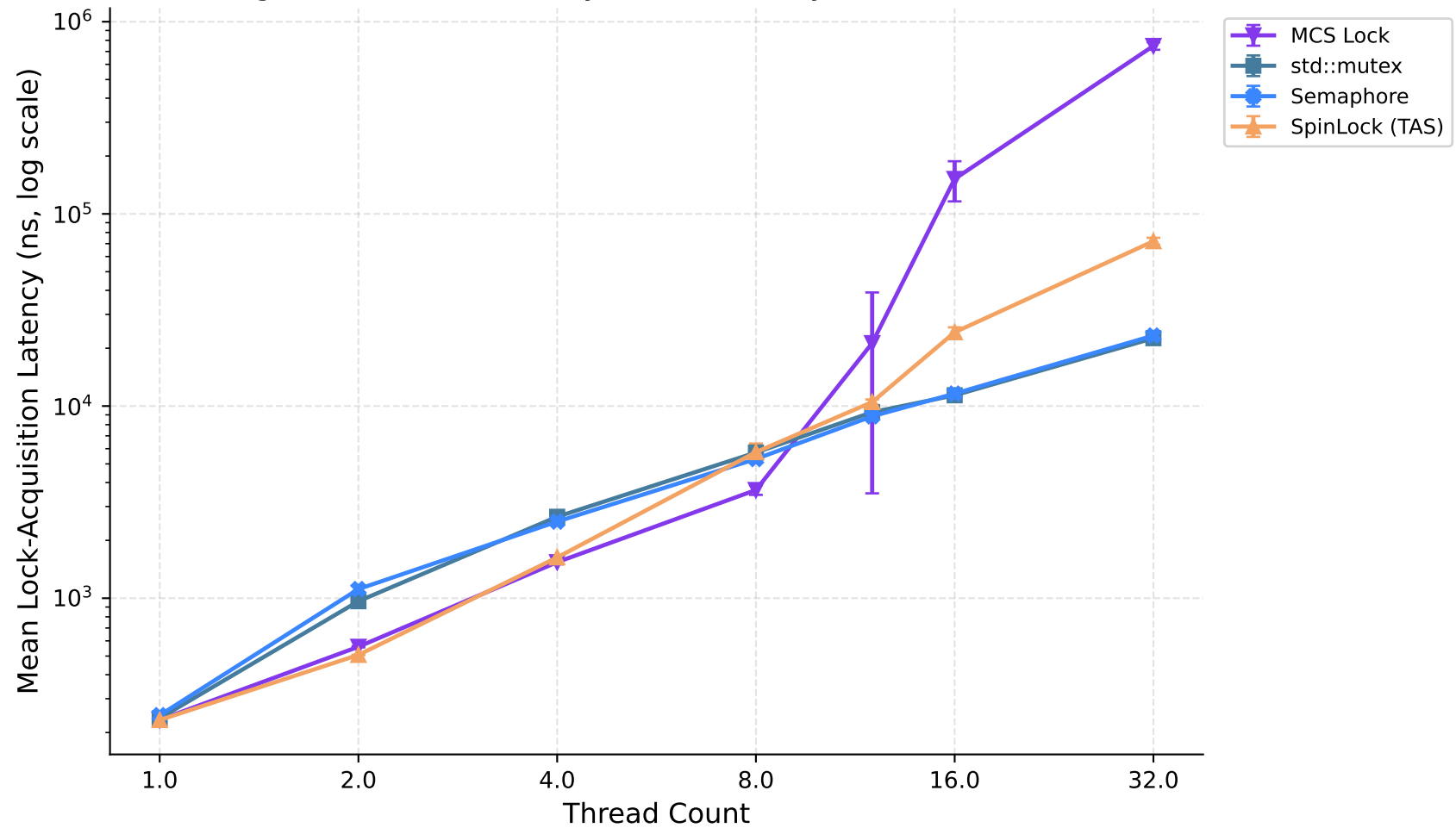
Fig 02 — Lock Scalability: Mean Latency vs Thread Count
