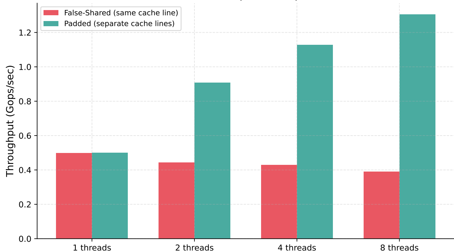
Fig 07 — False Sharing Effect (Same cache line vs padded separate lines)
