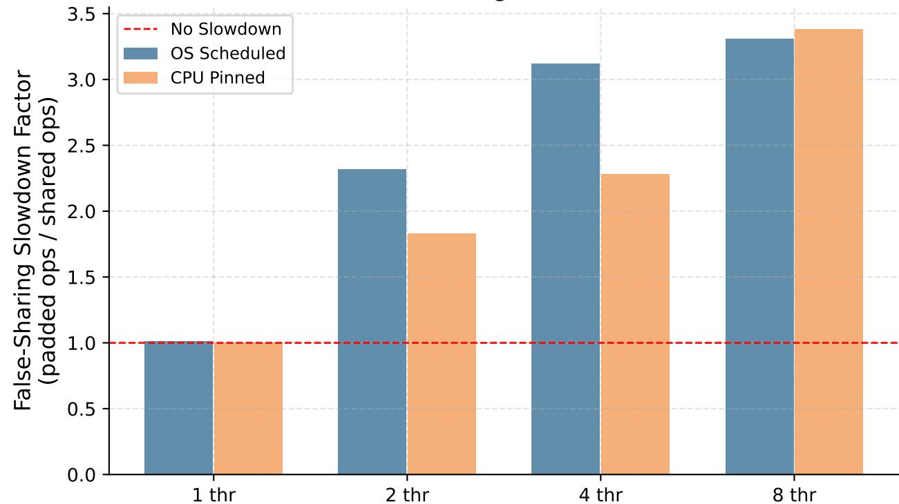
Fig 08 — Cache Line False-Sharing Slowdown Factor ( >1 = false sharing causes slowdown)
