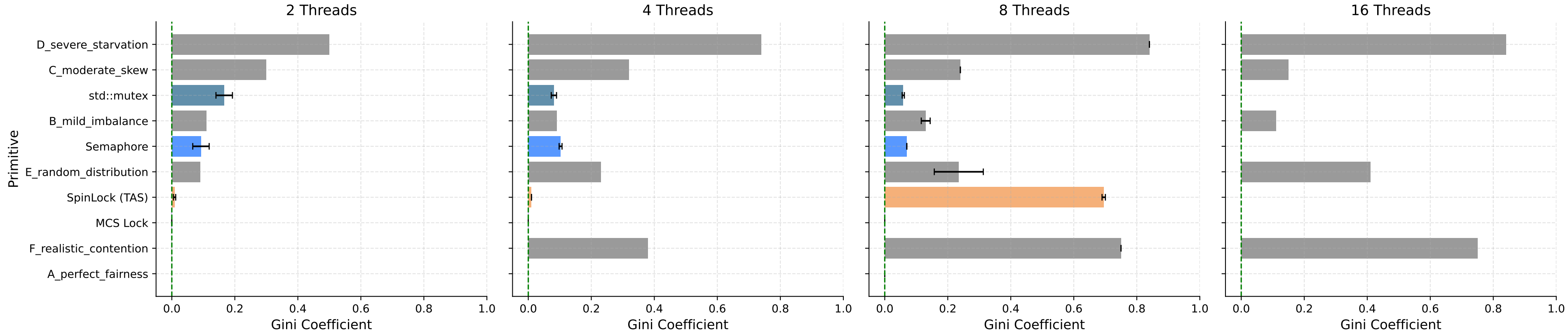
Fig 09 — Lock Fairness: Gini Coefficient (0 = perfect fairness, 1 = maximum starvation)
