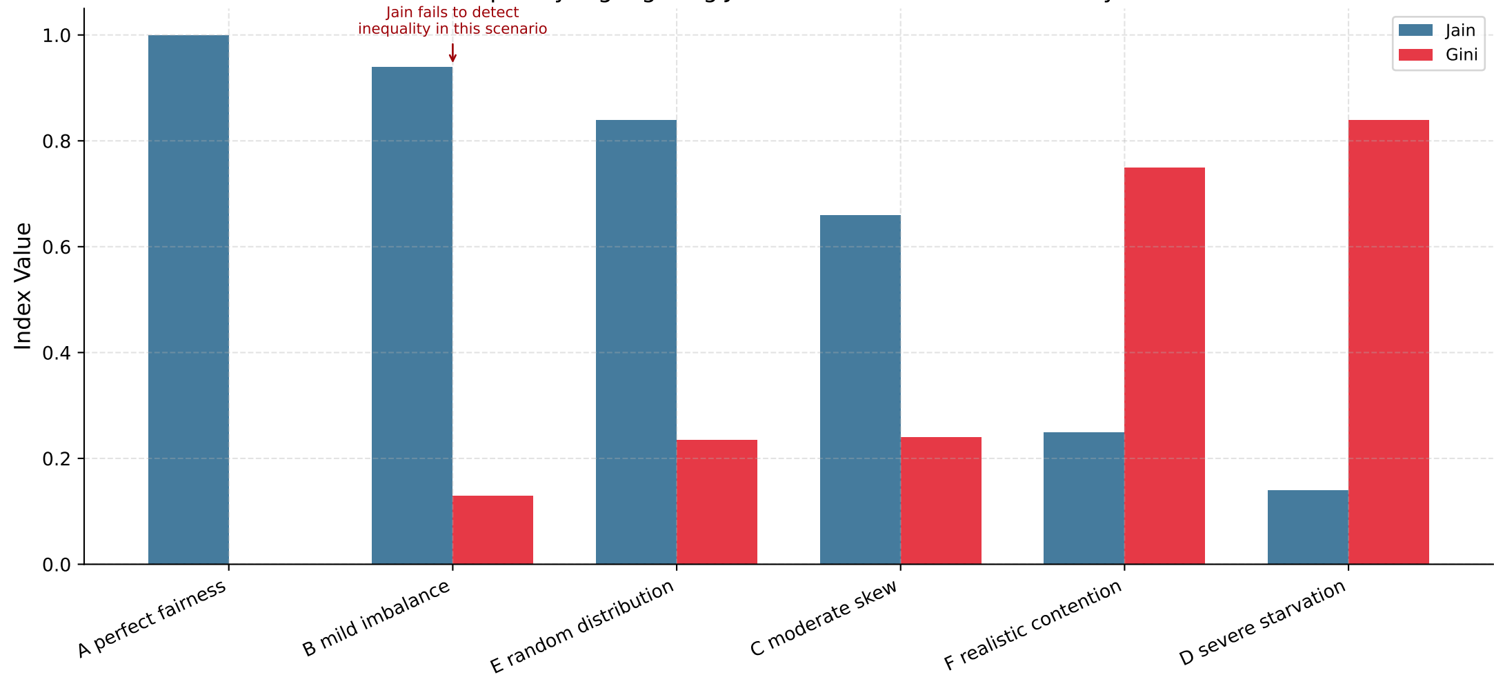
Fig 09c — Controlled Synthetic Scenarios (8 Threads): Jain vs Gini Explicitly highlighting Jain saturation vs Gini sensitivity
