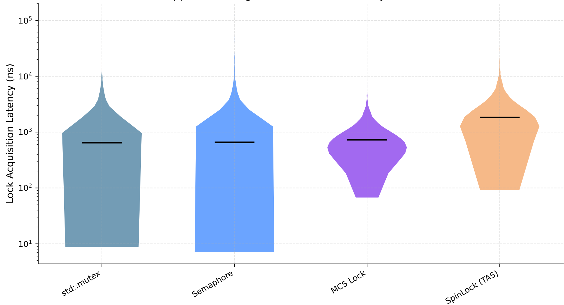
Fig 10 — Latency Distribution (Violin Plot) Approximate log-normal fit from summary statistics
