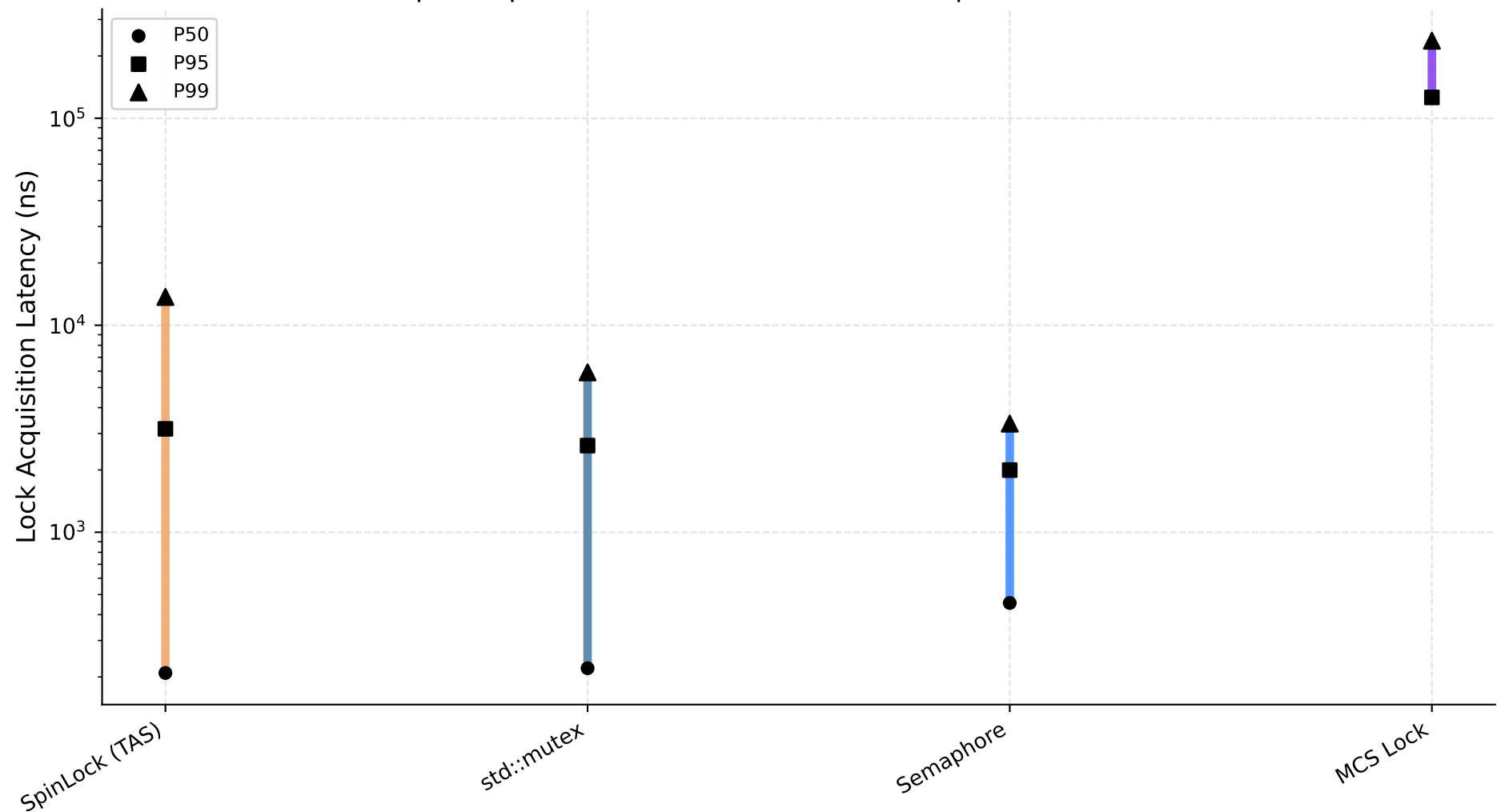
Fig 10 — Latency Quantile Interval Plot Empirical percentiles from benchmark output (not KDE/violin)
