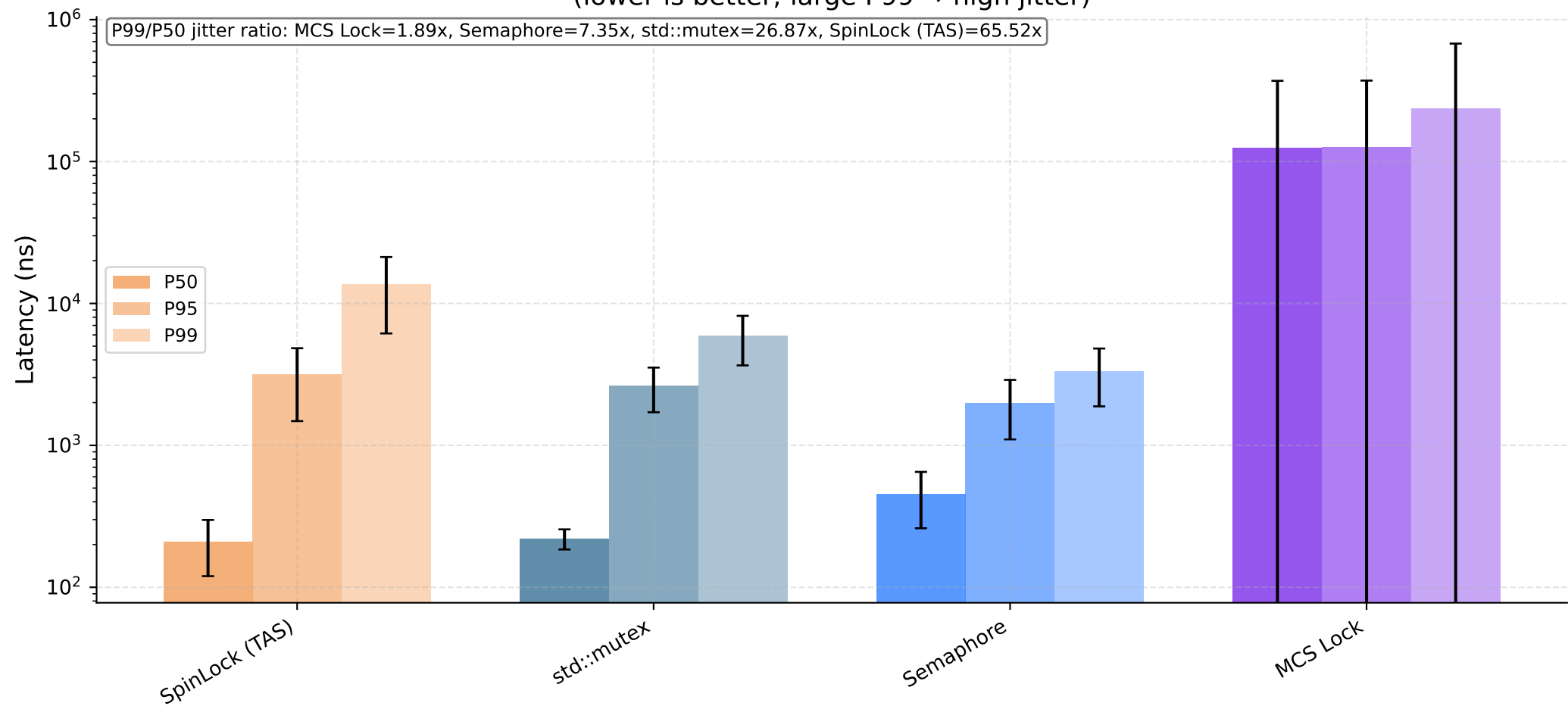
Fig 11 — Tail Latency Comparison: P50 / P95 / P99 (lower is better; large P99 → high jitter)
