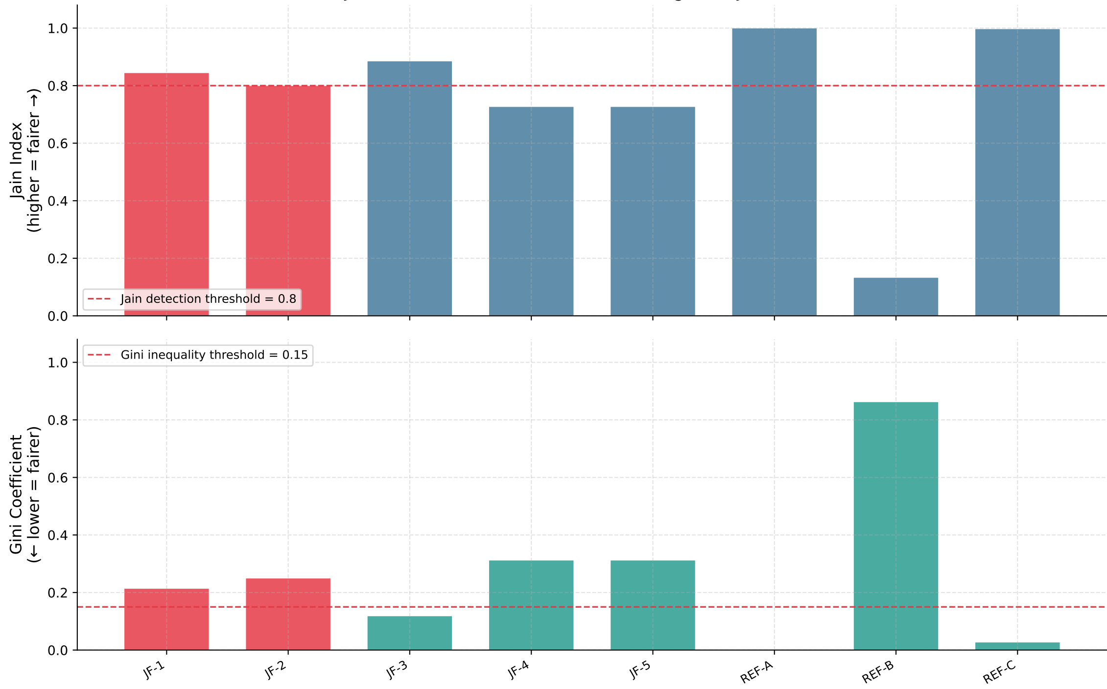
Plot E — Metric Comparison: Separate Panels with Explicit Polarity Red Jain bars = scenarios with metric divergence ( J \geq 0.80 , G \geq 0.15 )
