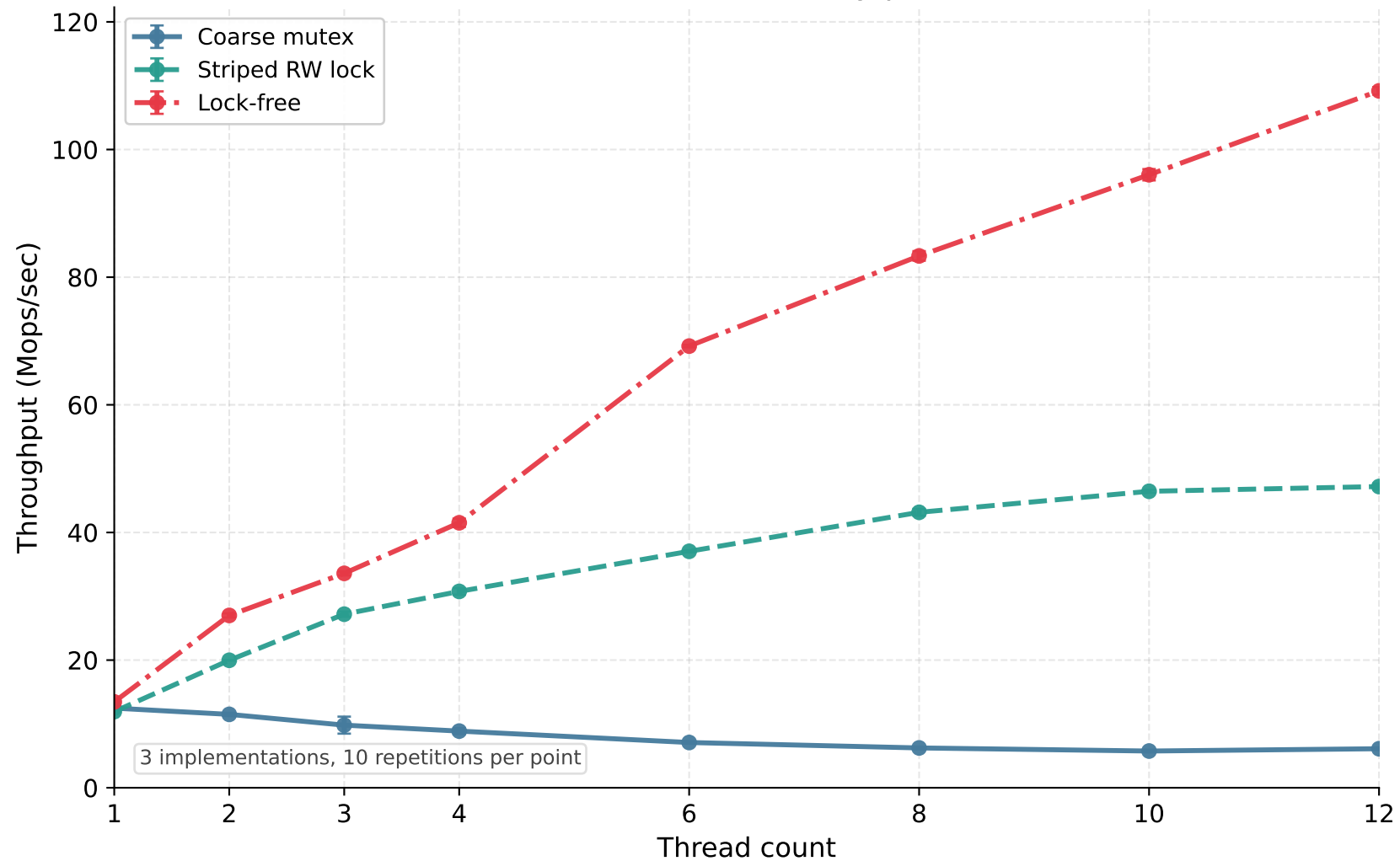
Concurrent Hash Table - Bursty phase behavior
