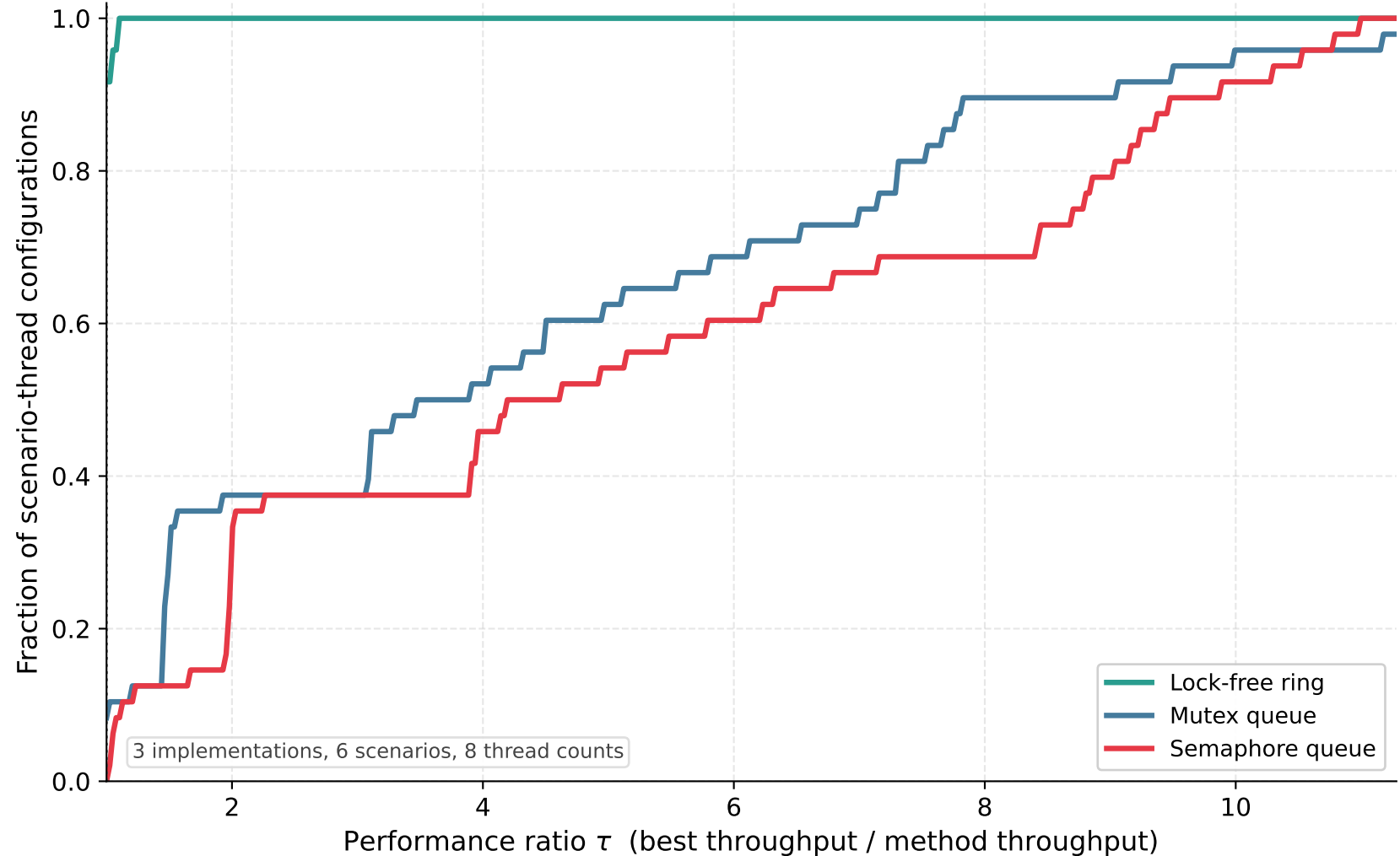
Bounded Producer-Consumer Queue - Performance Profile
