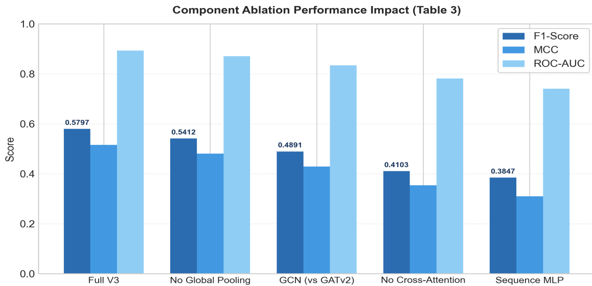
Fig. 4. Component ablation impact on F1, MCC, and ROC-AUC metrics across model variants.
