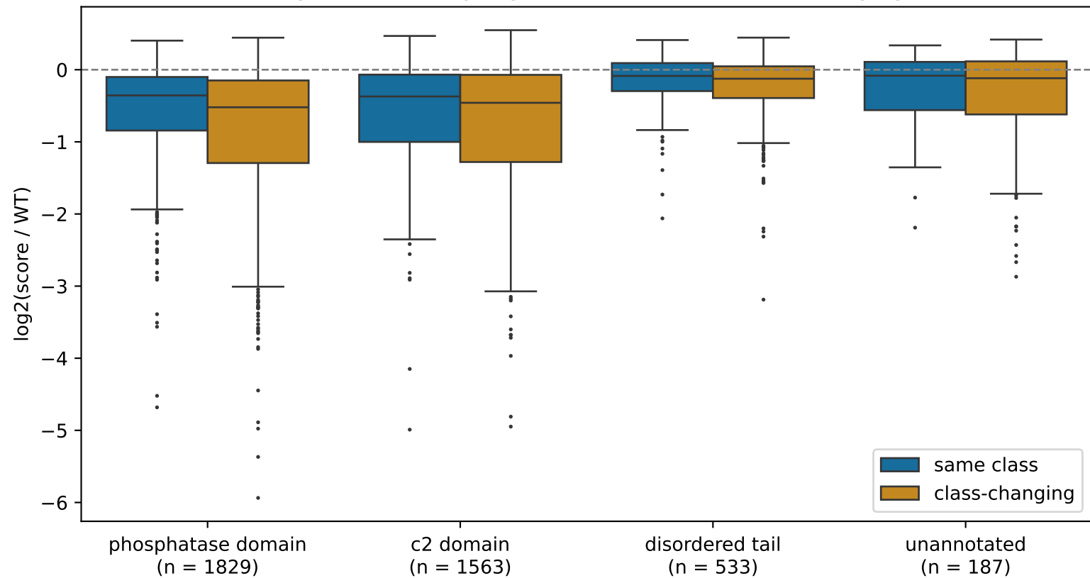
Log ratio to WT by region, same-class vs class-changing
