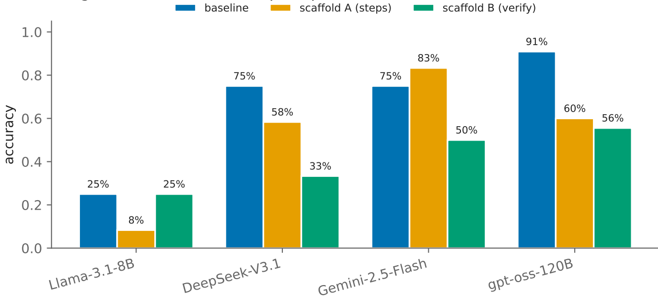
Mitigation: baseline vs two prompt scaffolds
