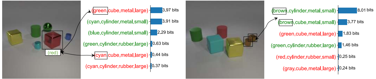
Figure 4. CLEVR examples of object-code uncertainty revealed by binding probes. Blue bars ( H(O|Z) ) indicate uncertainty in predicting objects. Left: Color misattribution in binding. Right: Uncertainty on the joint presence of a brown cylinder and a brown cube.
