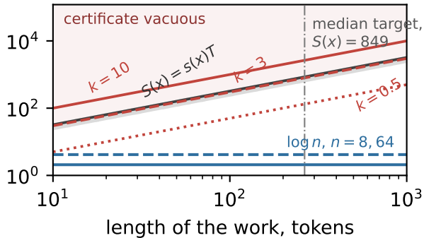
(c) kT grows with the work; \log n does not
