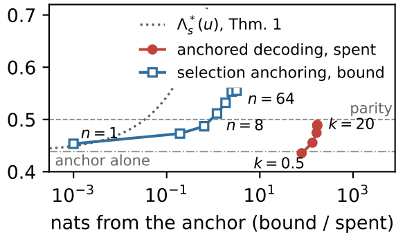
(d) what a nat buys, one judge, one opponent
